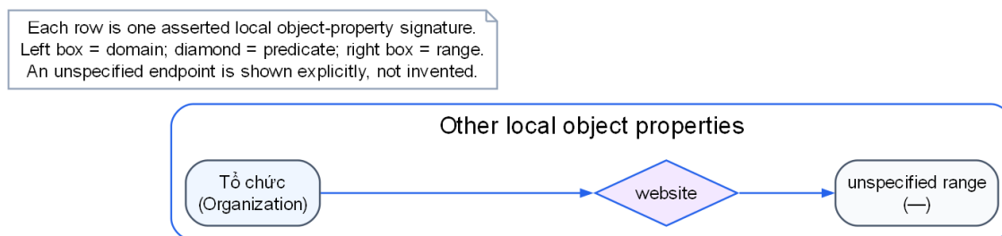
Figure 16: The remaining local object property, website , has an asserted domain but no asserted range in the ontology. This is shown as an open endpoint, not silently assigned xsd:anyURI .
