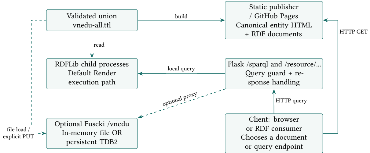
Figure 22: Publication and storage paths. The optional Fuseki branch has verified Linux and Windows acceptance runs; Render still explicitly selects local RDFLib. Storage does not replace the canonical identifiers.
