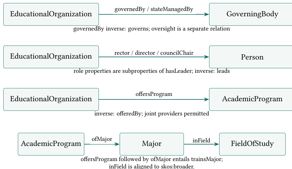
Figure 19: Selected domain-property-range signatures. These arrows are not mandatory foreign keys. Program providers and majors are no longer functional: multiple values must not force different institutions or subjects to become identical.
