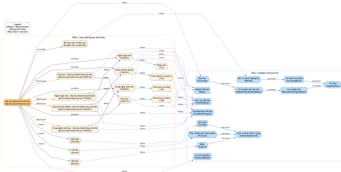
Figure 17: Data-driven ABox view generated from the gold serving union. The orange nodes are named individuals: one university, four programmes, four majors, four fields, location units and the reported governing body. Coloured edges are asserted or materialized object-property links; dashed rdfs:type edges connect only the most specific visible types to the TBox. This reproducible diagram supplements, but does not replace, the direct Protégé and GraphDB UI screenshots.
