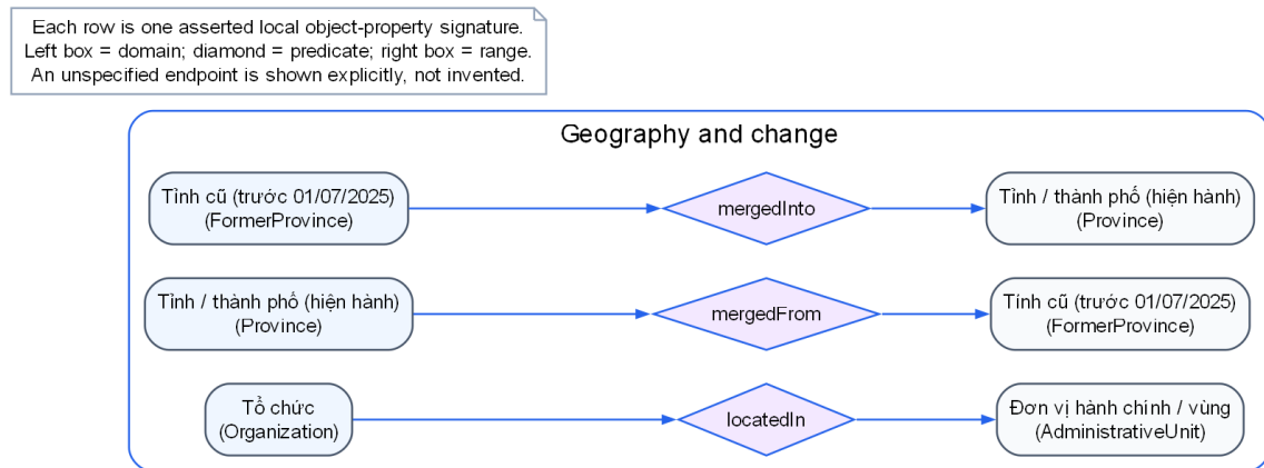
Figure 15: Exact local signatures for location and province-change relations. The former/current province distinction is represented as a directed relation, not as a timeless equivalence.
