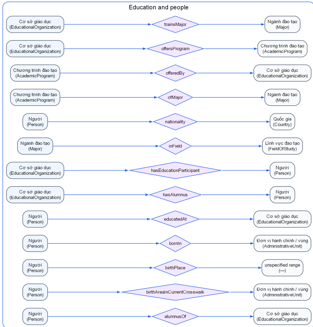
Figure 14: Exact local object-property signatures for programmes, majors, fields, people and educational participation. The missing range of birthPlace is shown explicitly as unspecified rather than guessed.
