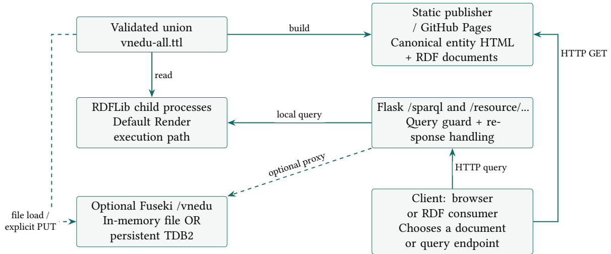
Figure 17: Publication and storage paths. The optional Fuseki branch has verified Linux and Windows acceptance runs; Render still explicitly selects local RDFLib. Storage does not replace the canonical identifiers.
