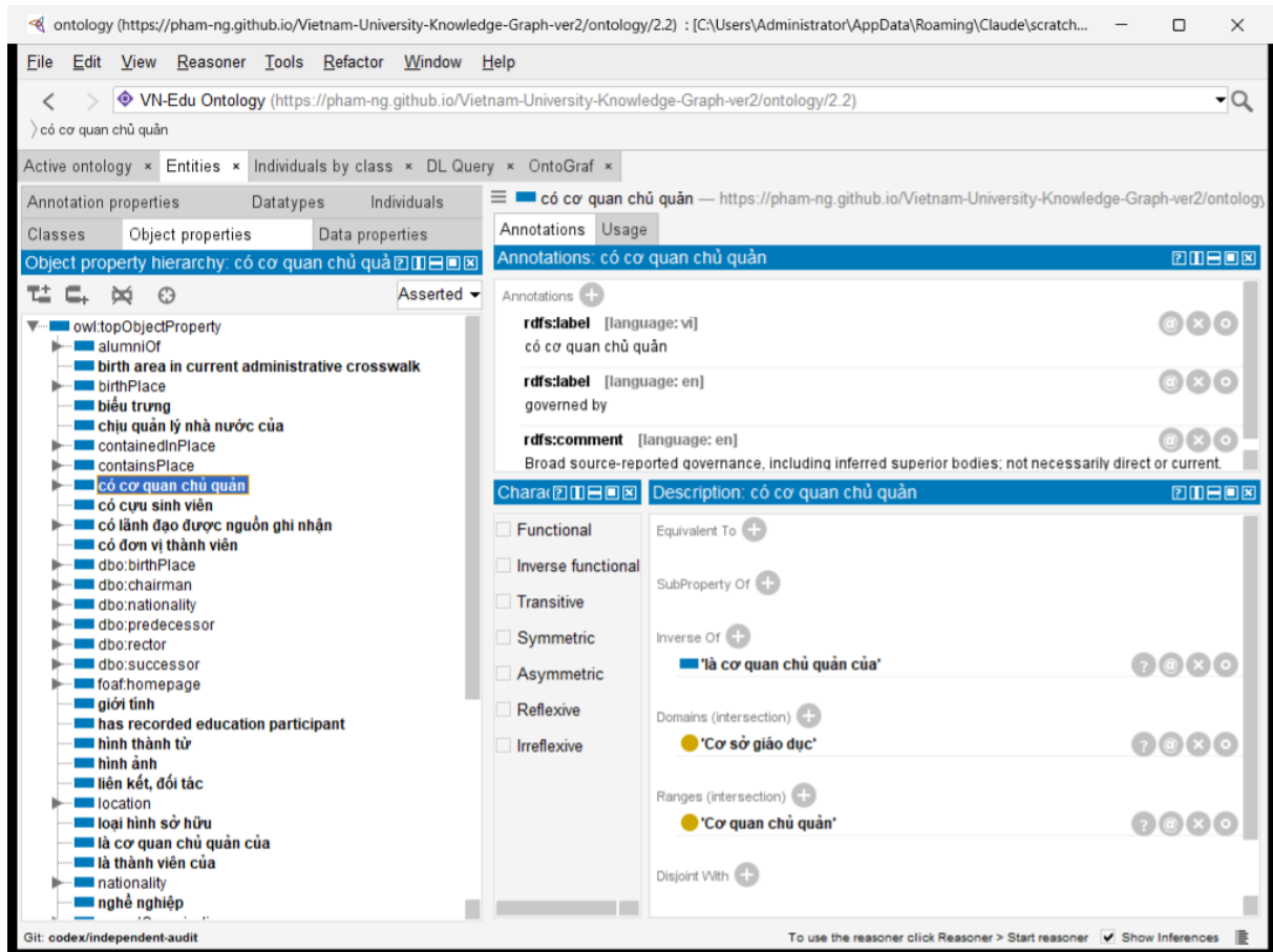
Figure 5: Direct screenshot of Protégé’s Object properties view for the committed ontology. The selected governedBy relation is displayed with bilingual labels, its comment, domain EducationalOrganization, range GoverningBody, and its inverse relation. This is the property-signature view used to verify that the graph has database-like domain–relationship–range discipline; it is not a hand-drawn diagram.
