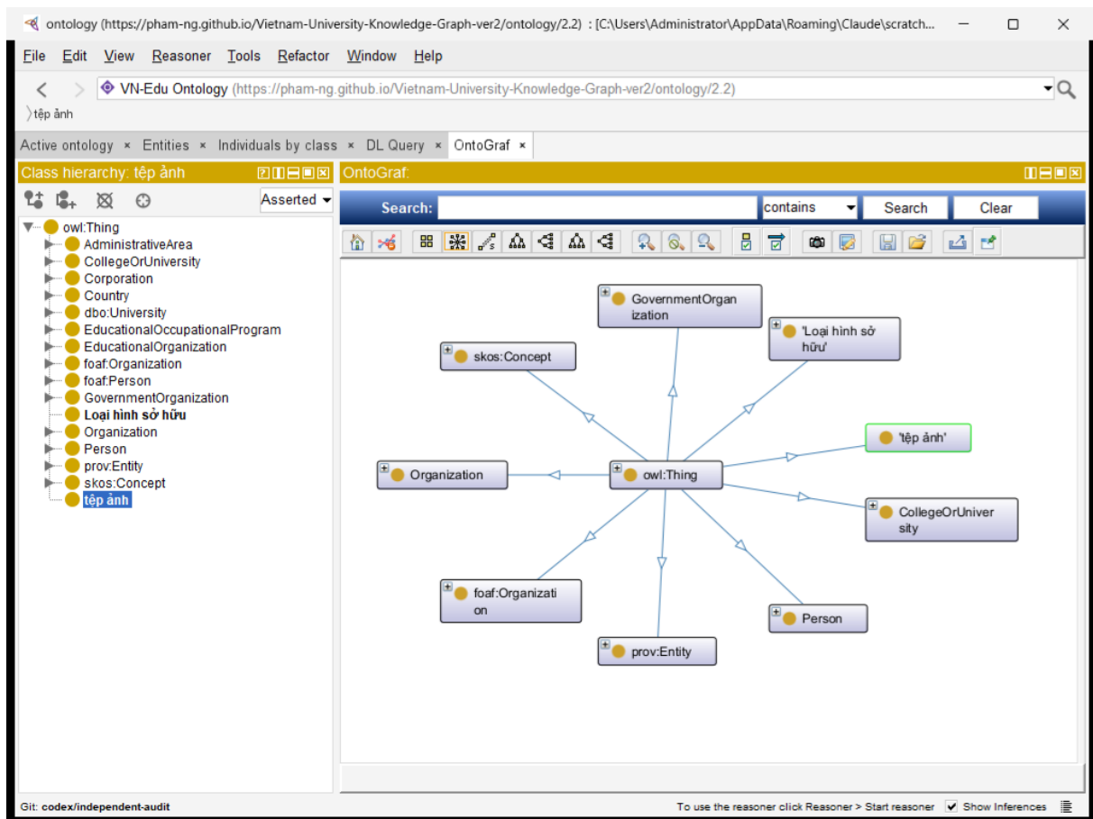
Figure 4: Direct screenshot of Protégé 5.6.7 with the OntoGraf plug-in, after loading the committed ontology/vnedu.ttl. The class hierarchy is shown at left and the selected ontology graph at right; the graph was laid out by OntoGraf and includes the selected OWL classes and their asserted subclass relations.
