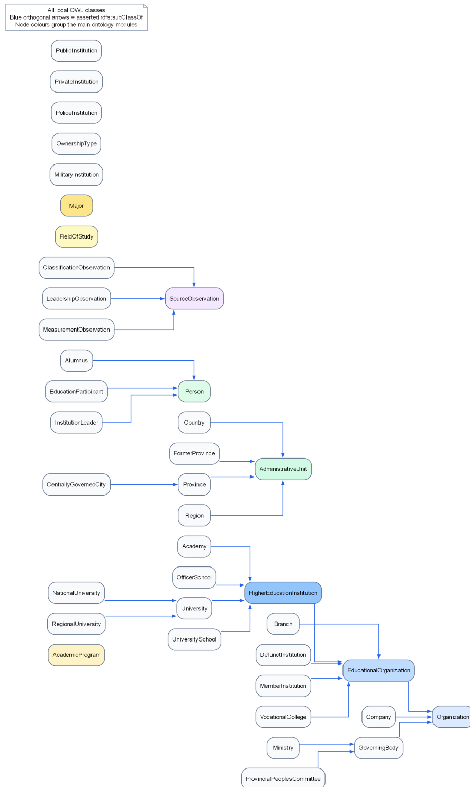
Figure 6: Complete local OWL class hierarchy generated directly from ontology/vnedu.ttl . Every displayed blue arrow is an asserted rdfs:subClassOf triple; disconnected nodes are intentionally retained because the ontology does not assert a superclass for them. Orthogonal routing is used to avoid crossing edges.
