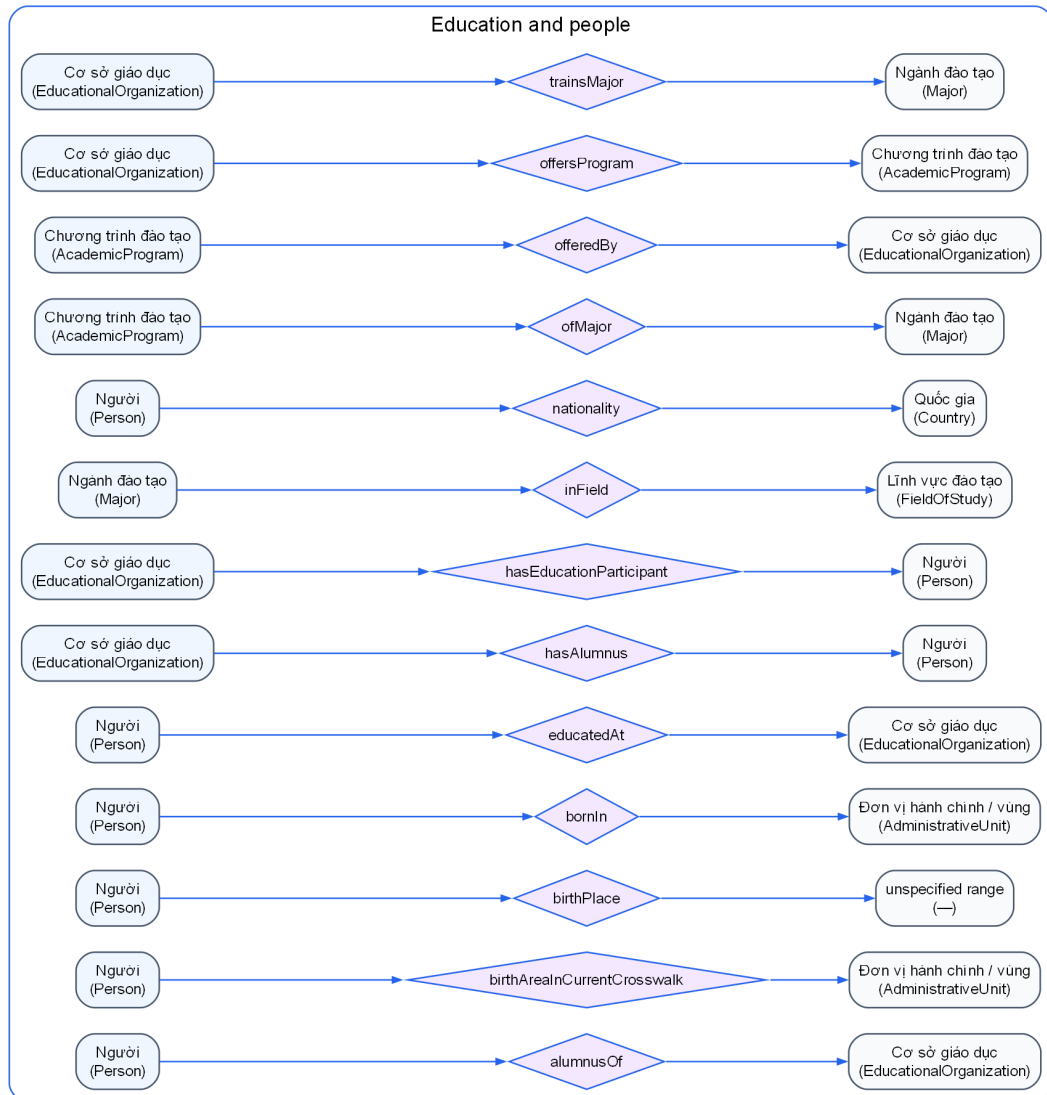
Figure 8: Exact local object-property signatures for programmes, majors, fields, people and educational participation. The missing range of birthPlace is shown explicitly as unspecified rather than guessed.
