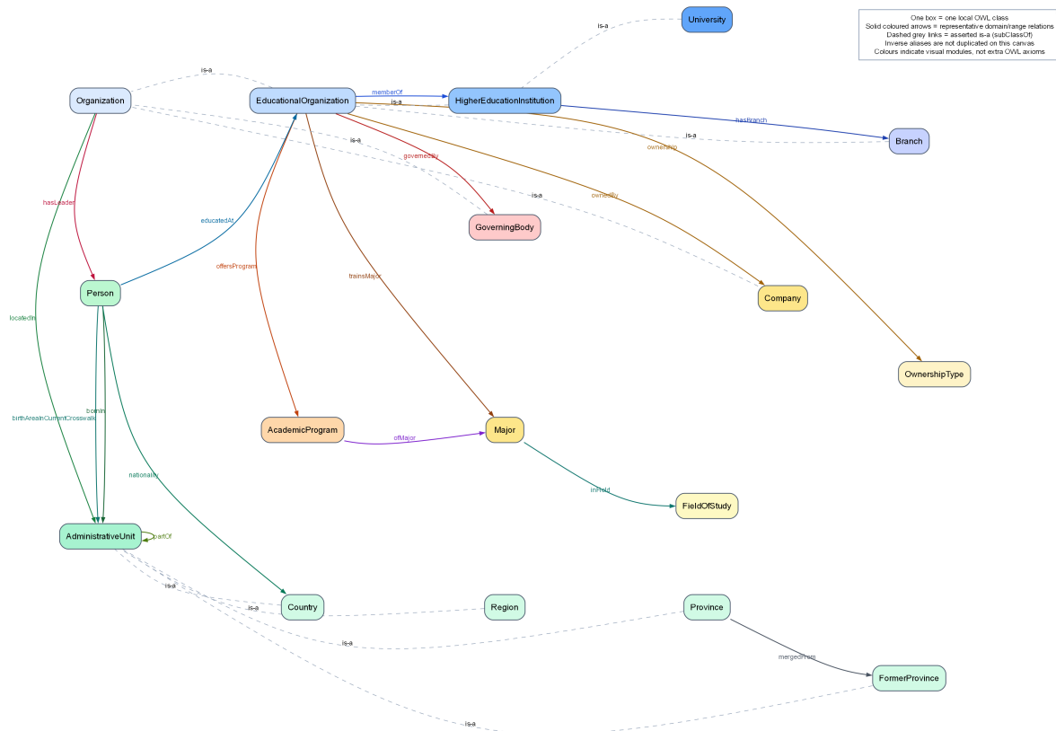
Figure 3: Main unique-node ontology map generated from the validated local OWL model. Each local class is rendered exactly once. Solid coloured arrows are asserted domain–range relations; dashed grey links are asserted rdfs:subClassOf axioms. The map uses one representative direction for inverse pairs so that it remains readable; the exact property inventory is documented separately. Coloured regions are presentation modules only and do not add OWL axioms.
