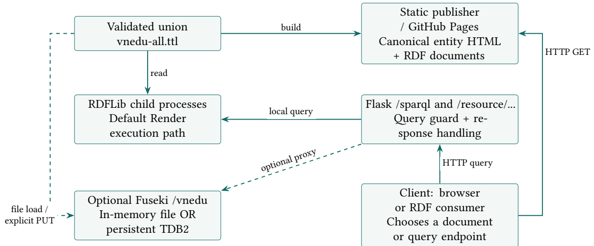
Figure 16: Publication and storage paths. The optional Fuseki branch has verified Linux and Windows acceptance runs; Render still explicitly selects local RDFLib. Storage does not replace the canonical identifiers.
