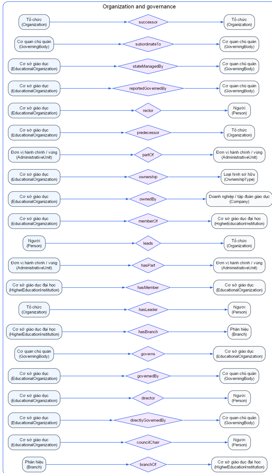
Figure 7: Exact local object-property signatures for organization, governance, membership, ownership and structural relations. Each row is independent: left box is the declared domain, the diamond is the predicate, and right box is the declared range. No edge is routed through another row.
