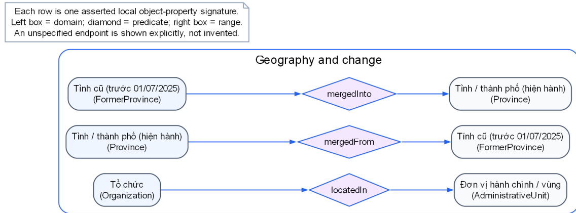
Figure 9: Exact local signatures for location and province-change relations. The former/current province distinction is represented as a directed relation, not as a timeless equivalence.
