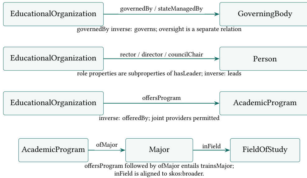
Figure 9: Selected domain–property–range signatures. These arrows are not mandatory foreign keys. Program providers and majors are no longer functional: multiple values must not force different institutions or subjects to become identical.
