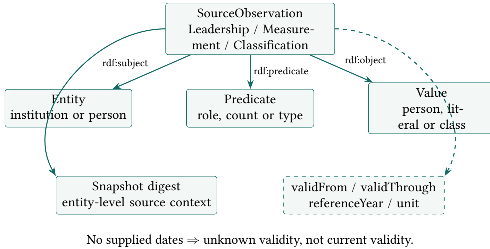
Figure 7: Observation model. Dashed fields are optional and must come from evidence. Missing dates mean unknown temporal validity. The diagram is schematic; no dates are fabricated for real officeholders.
