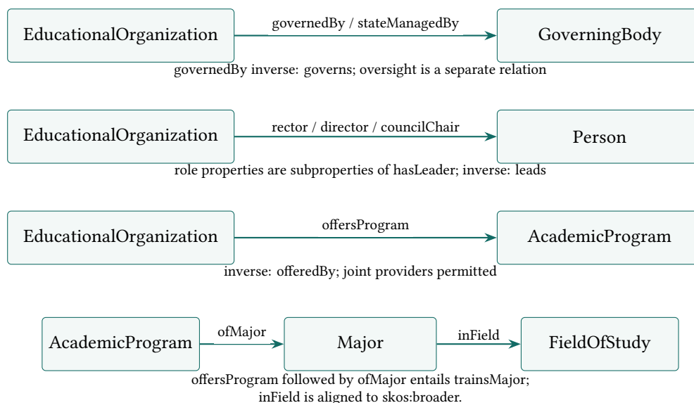
Figure 15: Selected domain-property-range signatures. These arrows are not mandatory foreign keys. Program providers and majors are no longer functional: multiple values must not force different institutions or subjects to become identical.
