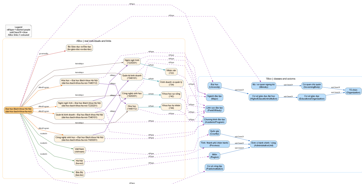
Figure 13: Data-driven ABox view generated from the gold serving union. The orange nodes are named individuals: one university, four programmes, four majors, four fields, location units and the reported governing body. Coloured edges are asserted or materialized object-property links; dashed rdfs:type edges connect only the most specific visible types to the TBox. This reproducible diagram supplements, but does not replace, the direct Protégé and GraphDB UI screenshots.
