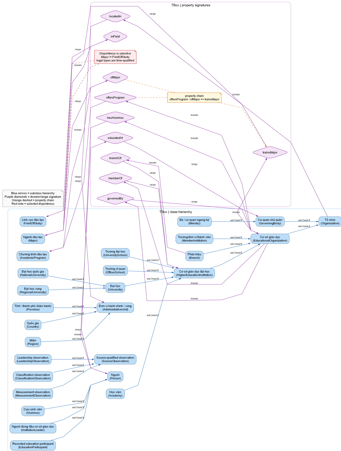
Figure 12: Data-driven TBox view generated from the committed ontology. The blue hierarchy shows multiple levels of specialization; purple diamonds make domain–property–range signatures explicit; the orange annotation records the offersProgram/ofMajor property chain that entails trainsMajor. The red annotation shows that disjointness is selective rather than a blanket rule over time-varying legal types.
