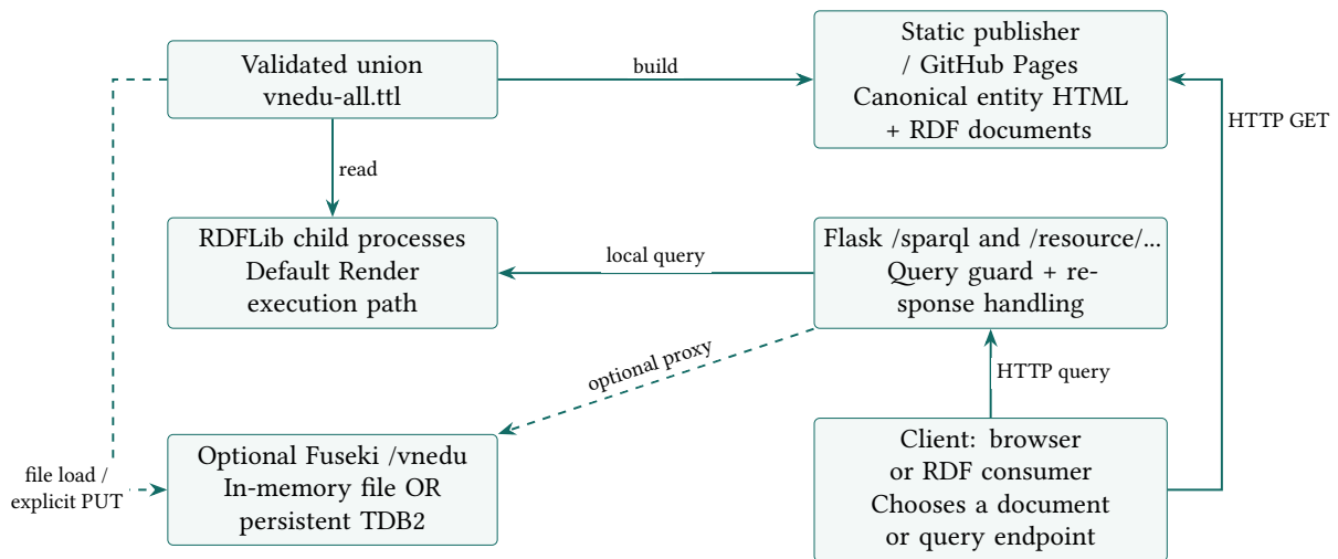
Figure 10: Publication and storage paths. The optional Fuseki branch has verified Linux and Windows acceptance runs; Render still explicitly selects local RDFLib. Storage does not replace the canonical identifiers.
