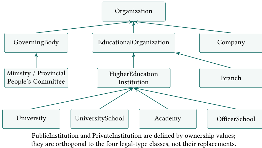
Figure 6: Selected organizational hierarchy. Arrows point from subclass to superclass. The four legal-type classes are no longer globally disjoint: an enduring institution can change type. This is a selected view of 39 classes.
