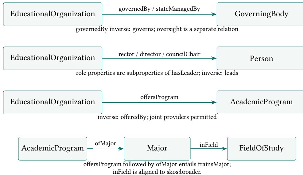
Figure 7: Selected domain-property-range signatures. These arrows are not mandatory foreign keys. Program providers and majors are no longer functional: multiple values must not force different institutions or subjects to become identical.
