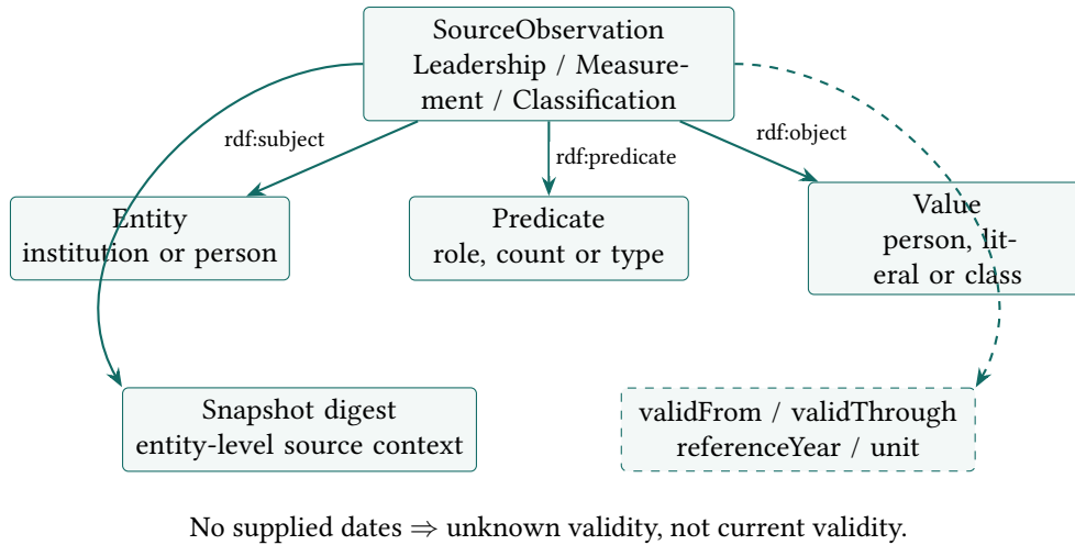
Figure 9: Observation model. Dashed fields are optional and must come from evidence. Missing dates mean unknown temporal validity. The diagram is schematic; no dates are fabricated for real officeholders.
