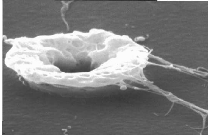
Figure 2-4 Electromigration Damage
