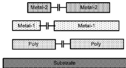
Figure 4-22 Sidewall Capacitance of Two Metal Route
