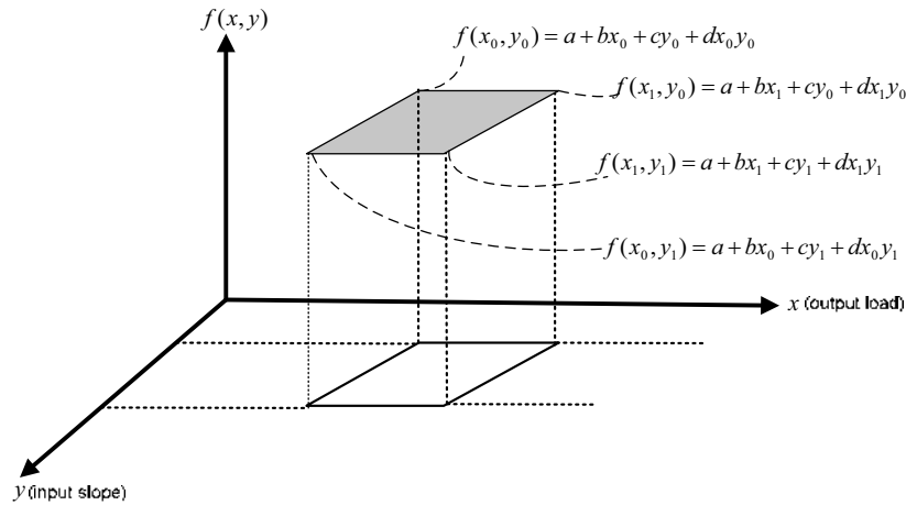
Figure 1-15 Nonlinear Delay Graph
