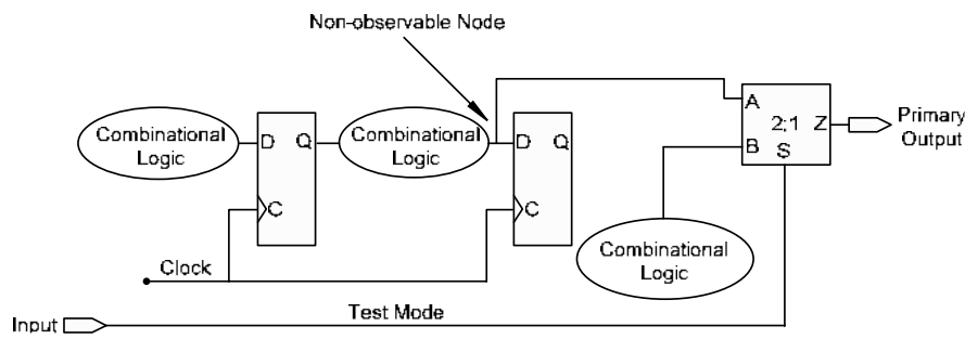
Figure 6-2 Non-observable Node
