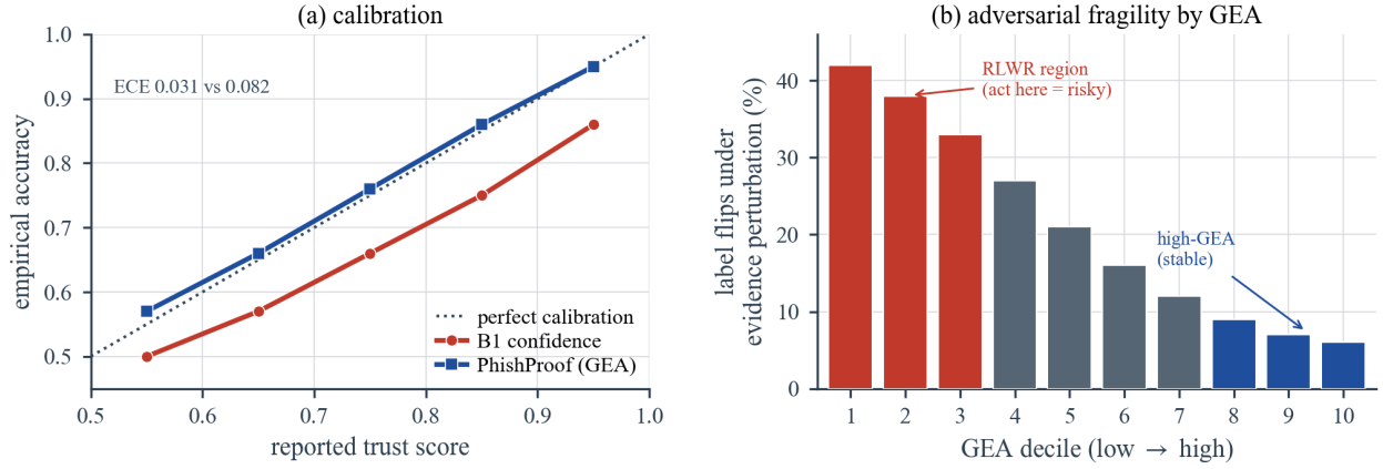
Figure 4: Diagnostics. (a) Calibrated trust tracks the diagonal while single-model confidence is over-confident. (b) Evidence-targeted label flips fall with GEA decile, showing that low-GEA/RLWR pages are fragile.
