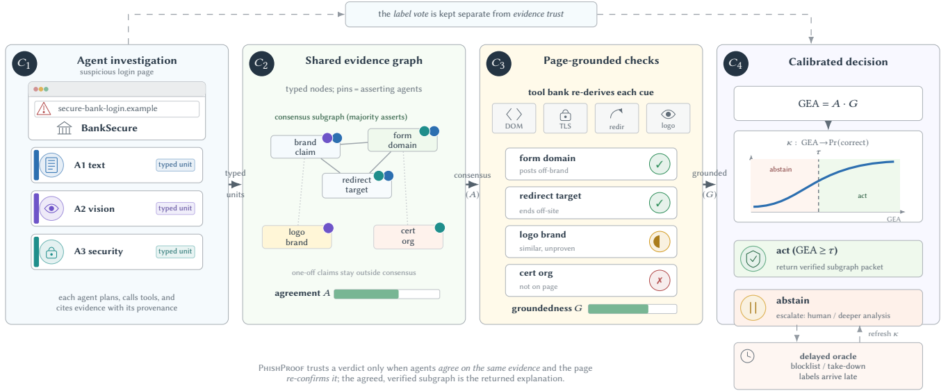
Figure 2: PHISHPROOF qualitative pipeline. Agents inspect the same page from complementary views, leave cited evidence notes, and place those notes on a shared evidence board. The system trusts a verdict only when the agents converge on the same page cues and the tool bank can re-check those cues against the live page. The calibrated selector returns the label with a verified evidence packet when the evidence is shared and grounded; otherwise it abstains, including cases where the label vote is plausible but the reasons are thin or unverified.
