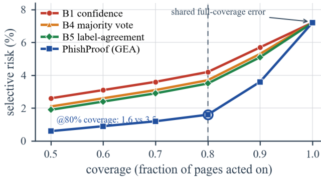
Figure 3: Risk-coverage on PHISHSEL (RQ1). Lower selective risk is better; the ring marks 80% coverage. PHISHPROOF changes the abstention order, not the majority label, and dominates across coverage.
