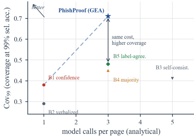
Figure 5: Cost-quality trade-off (RQ5): per-page model calls (analytical) versus coverage at 99% selective accuracy (Cov 99 , ↑). PHISHPROOF is Pareto-optimal – at the panel’s call budget it reaches the highest deployable coverage and dominates the label-level and self-consistency baselines.
