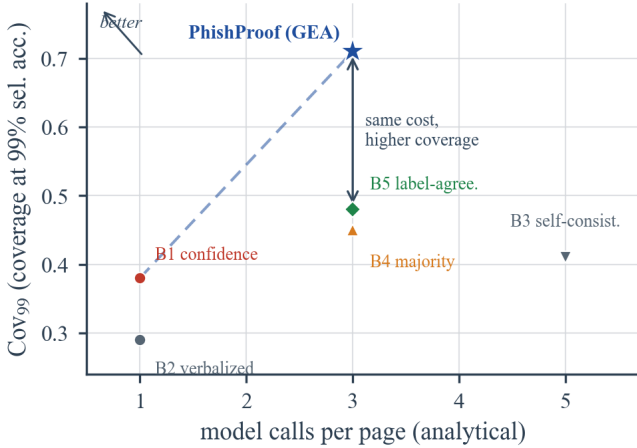
Figure 3: Cost-quality trade-off: per-page model calls (analytical) versus coverage at 99% selective accuracy ( Cov_{99} , \uparrow ). PHISHPROOF is Pareto-optimal – at the panel’s call budget it reaches the highest deployable coverage and dominates the label-level and self-consistency baselines.
