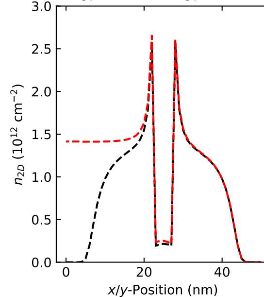
c) V_{34} = 0.0 V and V_{G4} = -5.0 V
