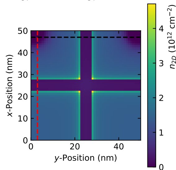
b) V_{34} = 0.0 V and V_{G4} = -5.0 V
