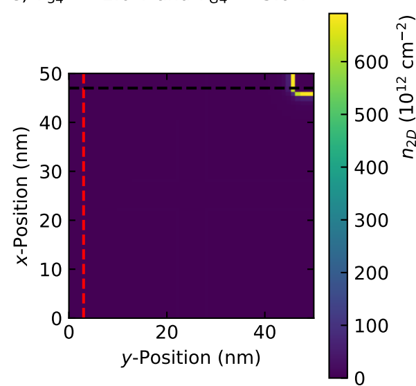
e) V_{34} = -2.0 V and V_{G4} = -5.0 V
