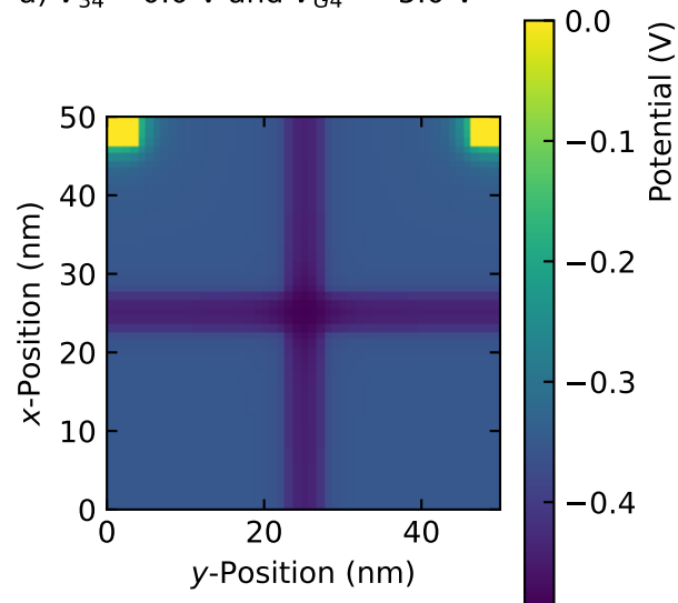
a) V_{34} = 0.0 V and V_{G4} = -5.0 V
