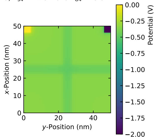
d) V_{34} = -2.0 V and V_{G4} = -5.0 V
