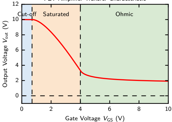
FET Amplifier Transfer Characteristic
