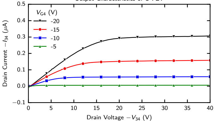
Output Characteristics of O-FET
