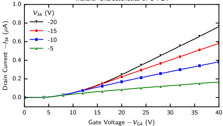
Transfer Characteristics of O-FET
