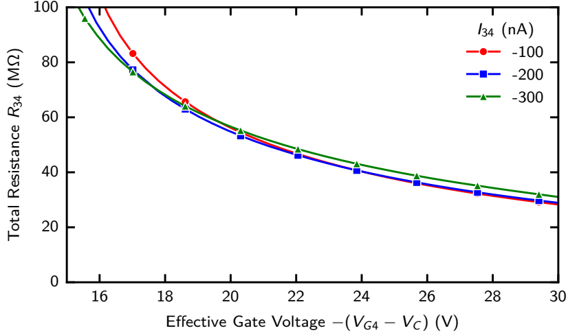
Figure 4.8: Total resistance R_{34} = |V_{34}/I_{34}| versus effective gate voltage V_{\text{eff}} = -(V_{G4} - V_C) for three imposed currents. The resistance decreases with increasing V_{\text{eff}} , and the three current series nearly overlap, with a small upward shift for the -300 nA series at larger V_{\text{eff}} .
