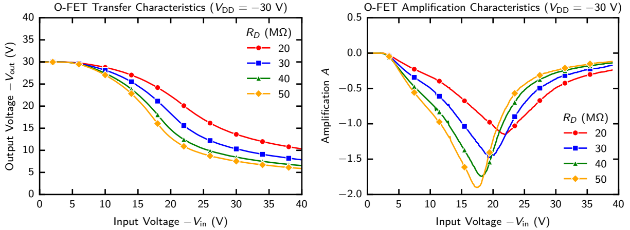
Figure 4.13: OFET transfer curve and amplification characteristic at V_{DD} = -30 V for different drain-load resistances R_D . The transfer plot identifies the input-voltage range where the output voltage changes most strongly, while the amplification plot shows the corresponding small-signal voltage gain. Larger R_D values increase the maximum gain but also narrow the useful operating range.
