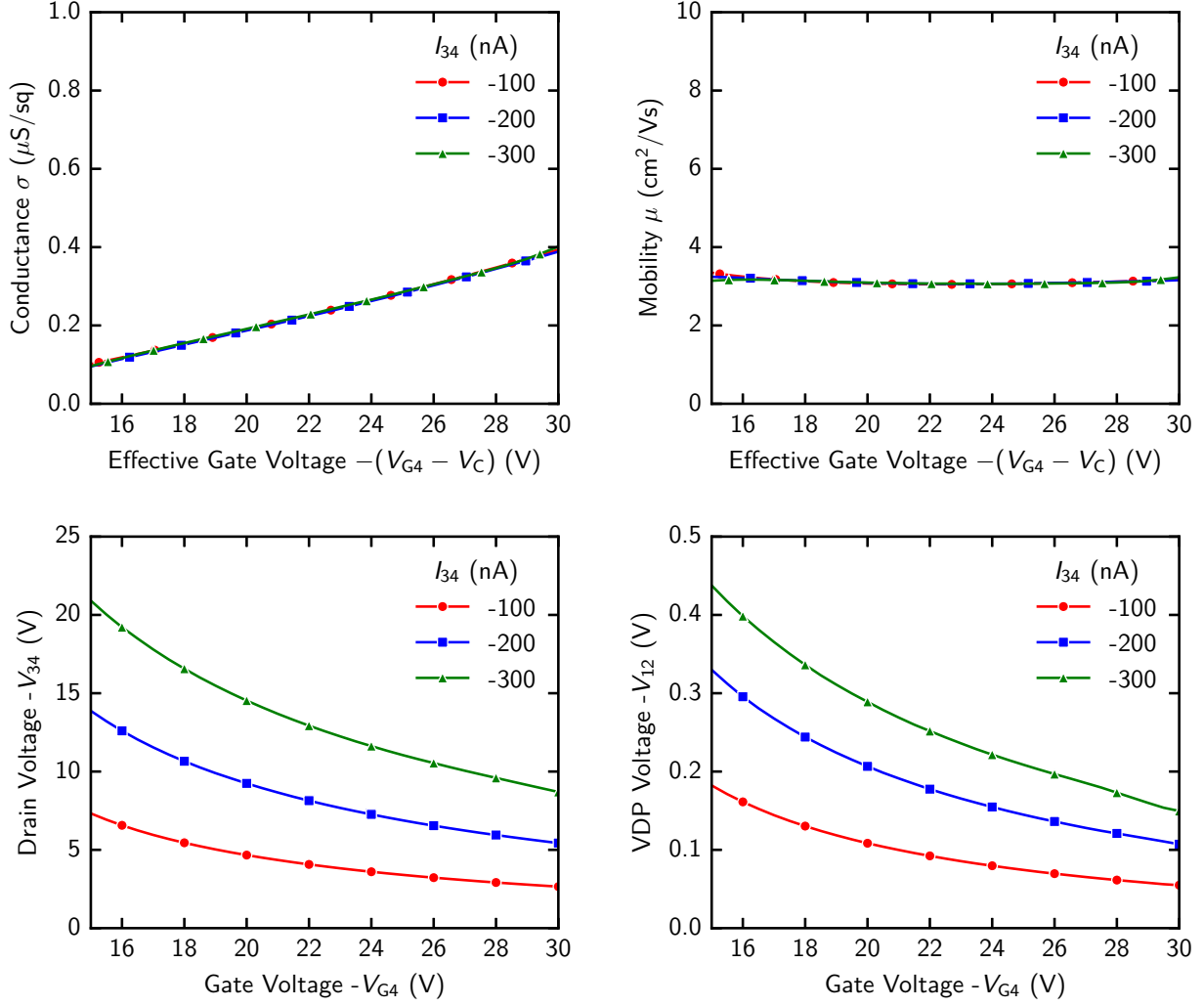
Figure 4.7: Gated van der Pauw extraction for I_{34} = -100 nA, -200 nA, and -300 nA. The lower panels show the measured voltages, while the upper panels show the extracted sheet conductance \sigma and mobility versus effective gate voltage. The overlap of the three current series indicates linear-response behaviour and supports a current-independent mobility extraction.
