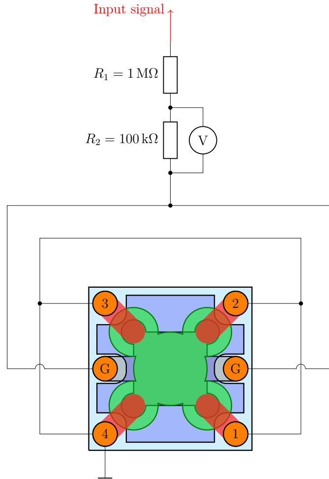
Figure 4.9: Circuit used for the deep-level transient spectroscopy (DLTS)-type measurements on the OFET structure. The external excitation is applied through the resistive divider formed by R_1 = 1\text{ M}\Omega and R_2 = 100\text{ k}\Omega . The voltage across R_2 is monitored so that the transient response of the device can be followed after each bias perturbation.
