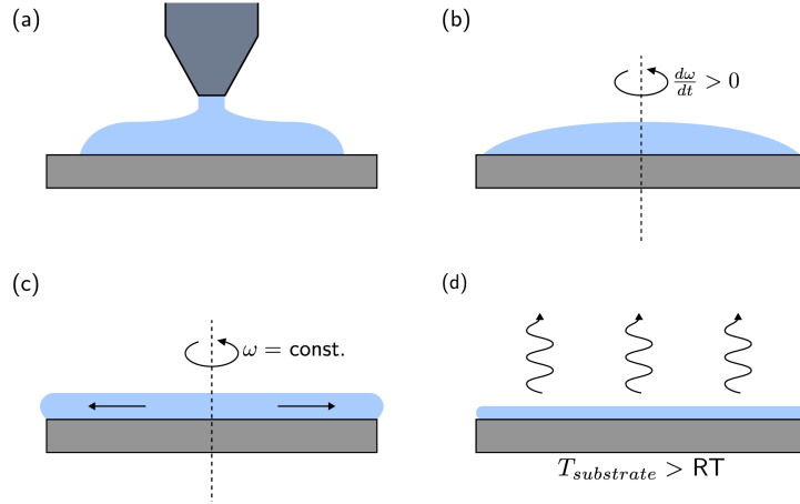
Figure 3.6: Schematic of the spin coating procedure. Figure from Ref. [Riederer2023Dissertation].
