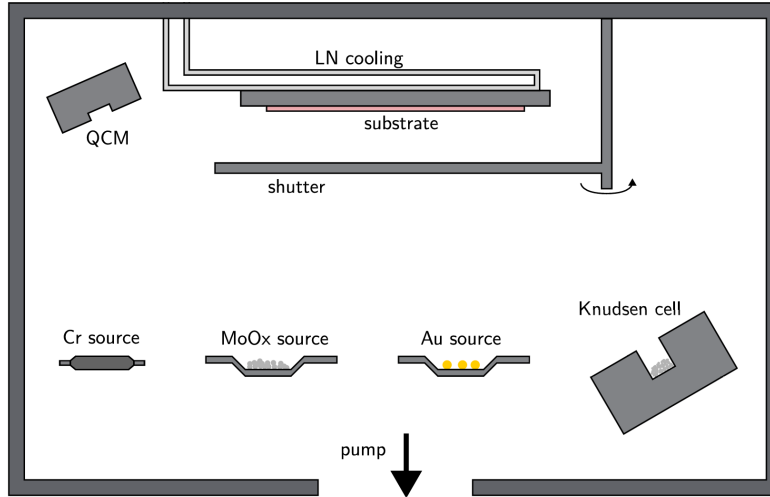
Figure 3.3: Schematic of the physical vapor deposition (PVD) system. Figure from Ref. [Riederer2023Dissertation].
