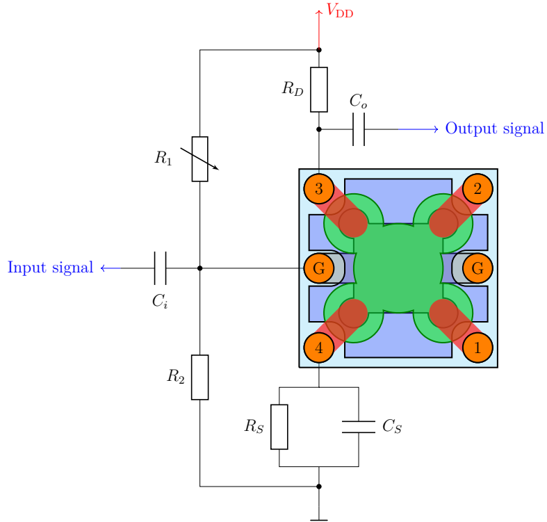
Figure 4.12: Circuit used to analyse the amplification properties of the OFET. The input signal is capacitively coupled to the gate through C_i = 1 nF, while the gate operating point is set by the bias divider with R_2 = 100 k \Omega and variable R_1 . The drain is biased through R_D at V_{DD} = -30 V, with R_D varied from 20 M \Omega to 50 M \Omega . The output signal is measured at the drain contact through C_o = 1 nF. The source branch contains R_S and the bypass capacitor C_S = 1 nF, which set the source bias and influence the small-signal response.
