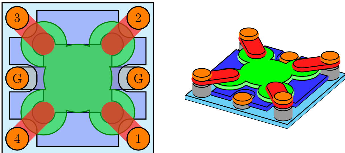
Figure 3.2: Schematic representation of the assembled OFET structure. The left panel shows the top-view contact layout, while the right panel shows the corresponding 3D layer structure. The central green region denotes the molecular semiconductor, the red diagonal paths indicate the four injection contacts, the orange pads provide external electrical access, and the side pads marked G connect to the bottom gate. Adapted from the figures in the internal laboratory archive.
