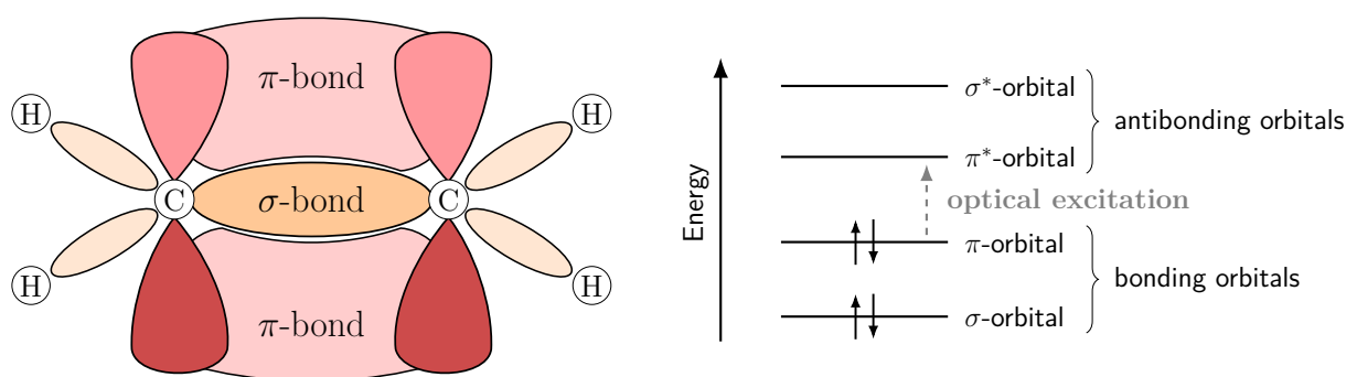
Figure 2.6: Sigma and pi bonding in ethene as the simplest conjugated pi-electron system. The left panel illustrates the spatial overlap of the \sigma and \pi bonds, while the right panel shows the corresponding bonding and antibonding orbital levels. The lowest optical excitation occurs from the bonding \pi orbital to the antibonding \pi^* orbital. Adapted from Ref. [Riederer2023Dissertation] and [Neamen].
