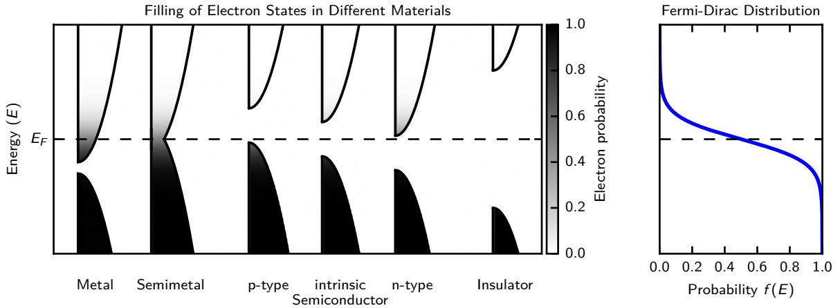
Figure 2.1: Electron occupancy of allowed energy bands in metals, semimetals, semiconductors, and insulators at temperature T > 0 \text{ K} . Shading indicates Fermi–Dirac occupation from filled states (black) to empty states (white).
