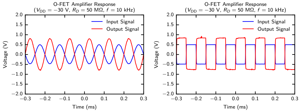
Figure 4.14: Dynamic response of the OFET amplifier at V_{DD} = -30 \text{ V} , R_D = 50 \text{ M}\Omega , V_{G,Q} = -18 \text{ V} , and f = 10 \text{ kHz} . The sinusoidal measurement demonstrates inverted voltage amplification, while the square-wave measurement shows the finite rise and fall times caused by the large circuit resistance, device capacitance, and trap-related relaxation.
