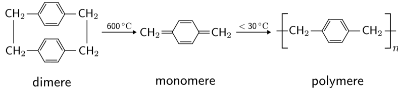
Figure 3.4: Schematic of the chemical synthesis of parylene-N (PaN). Figure from Ref. [Riederer2023Dissertation].
