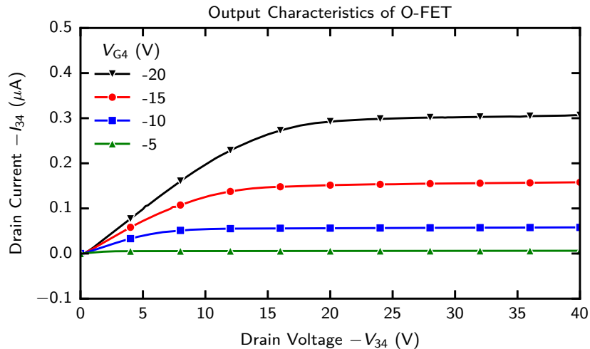
Figure 4.5: Output characteristic of the organic FET, measured as drain current -I_{34} as a function of drain voltage -V_{34} for different fixed gate voltages V_{G4} .
