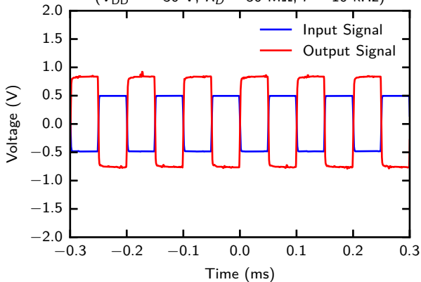
O-FET Amplifier Response ( V_{DD} = -30\text{ V} , R_D = 50\text{ M}\Omega , f = 10\text{ kHz} )
