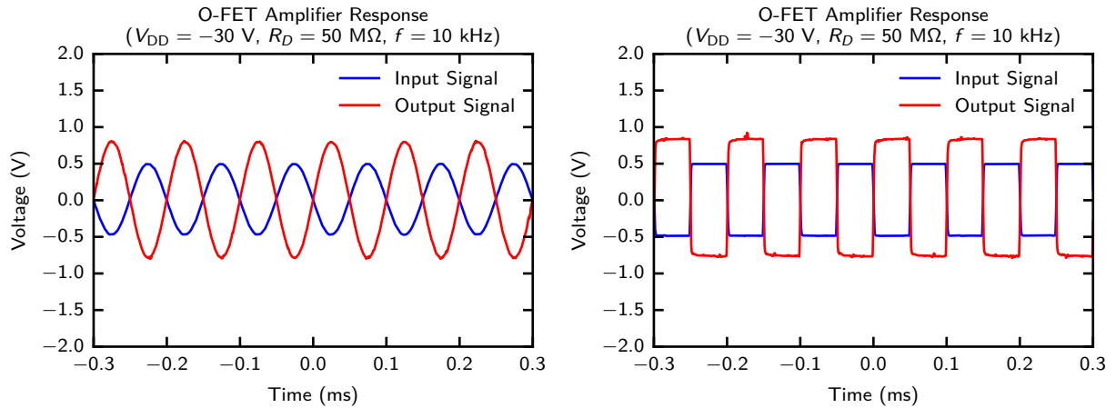
Figure 4.14: Dynamic response of the OFET amplifier at V_{DD} = -30 V, R_D = 50 M \Omega , V_{G,Q} = -18 V, and f = 10 kHz. The sinusoidal measurement demonstrates inverted voltage amplification, while the square-wave measurement shows the finite rise and fall times caused by the large circuit resistance, device capacitance, and trap-related relaxation.
