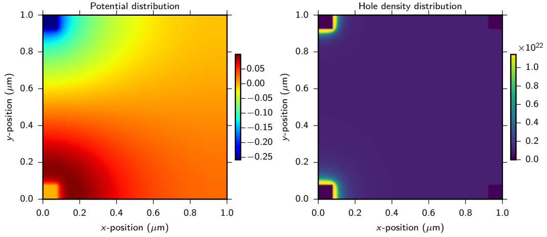
Figure C.1: Calculated potential and hole-density distributions in the lateral van der Pauw structure. The potential map is obtained by iteratively solving Poisson's equation on the two-dimensional grid with fixed contact potentials and insulating outer boundaries. The hole-density map is then calculated from the local electrochemical energy and shows hole accumulation near the current-carrying contacts.
