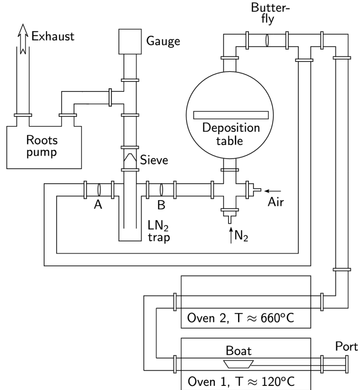
Figure 3.5: Schematic of the chemical vapor deposition (CVD) system used for PaN deposition. Figure from Ref. [Kersting2026FiguresCollection].
