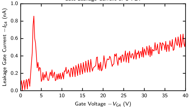
Gate Leakage Current of O-FET
