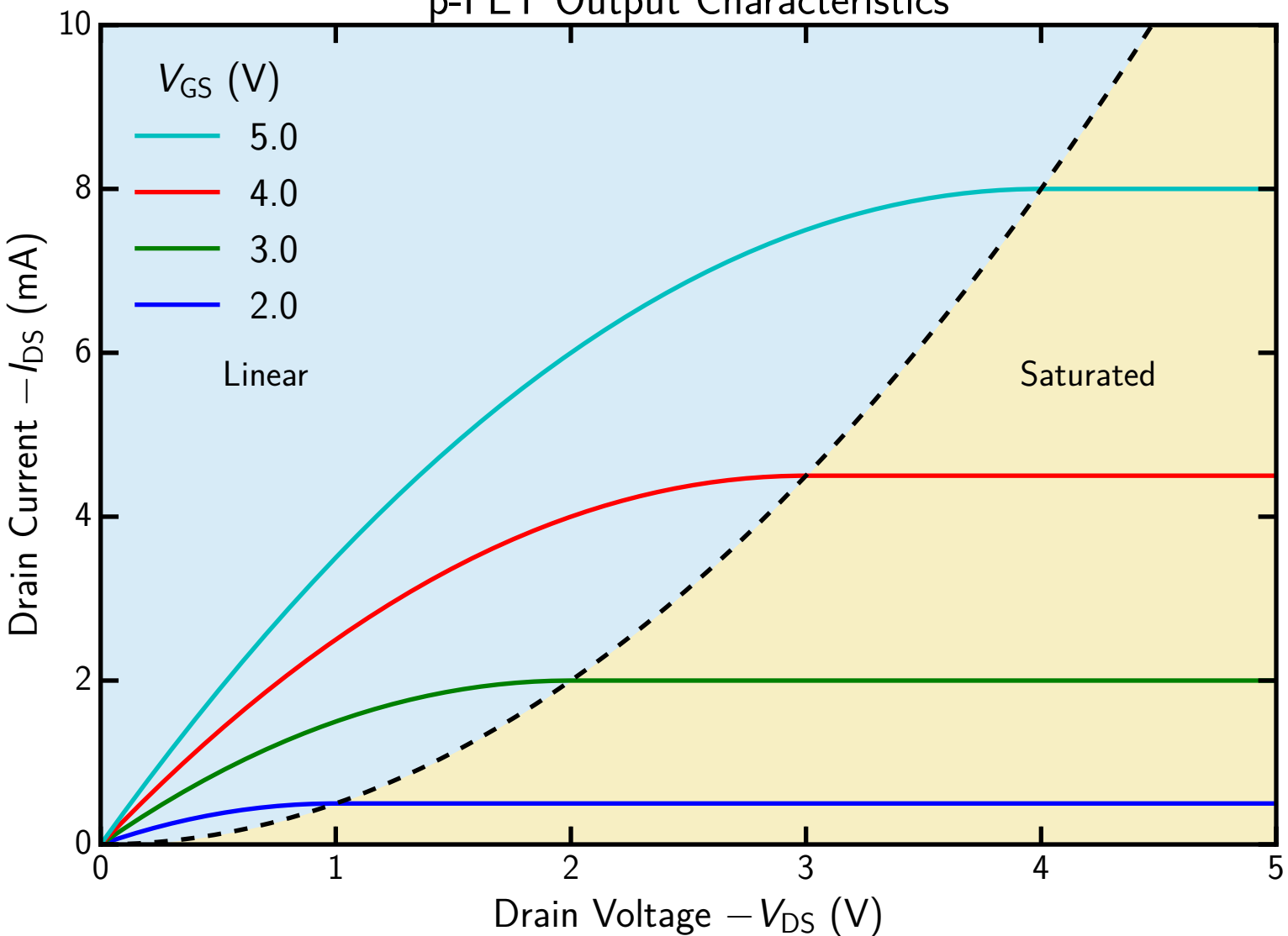
p-FET Output Characteristics
