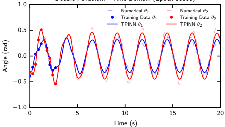
Double Pendulum - Time Domain (Epoch 30000)
