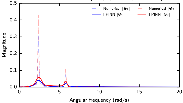
Double Pendulum - Frequency Spectrum (Epoch 1000)
