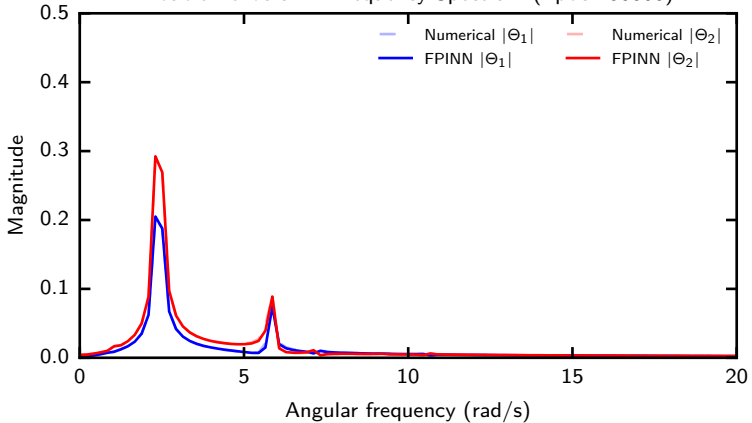
Double Pendulum - Frequency Spectrum (Epoch 50000)
