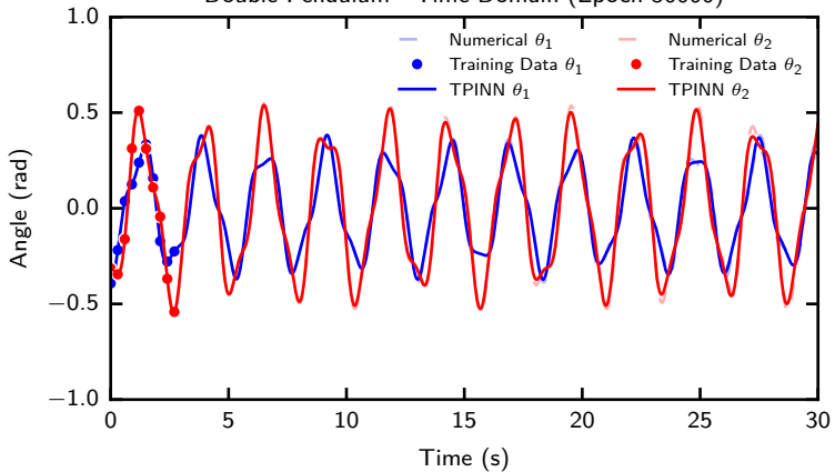
Double Pendulum - Time Domain (Epoch 50000)
