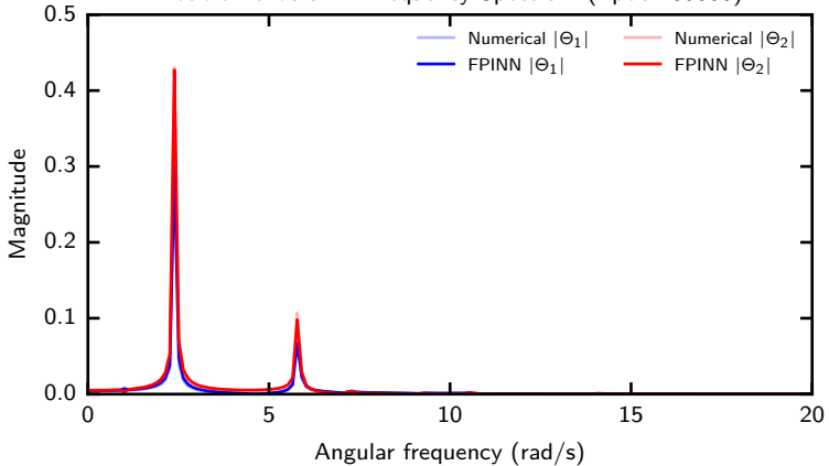
Double Pendulum - Frequency Spectrum (Epoch 30000)
