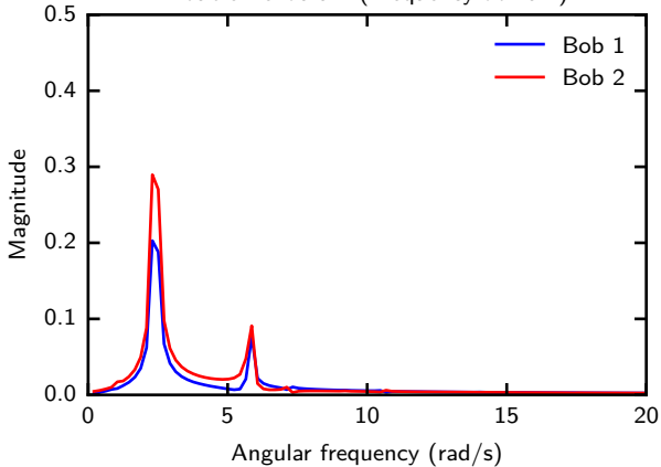
Double Pendulum (Frequency domain)
