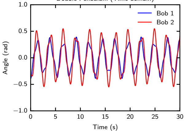
Double Pendulum (Time domain)
