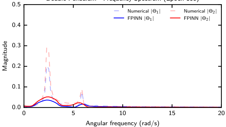
Double Pendulum - Frequency Spectrum (Epoch 100)
