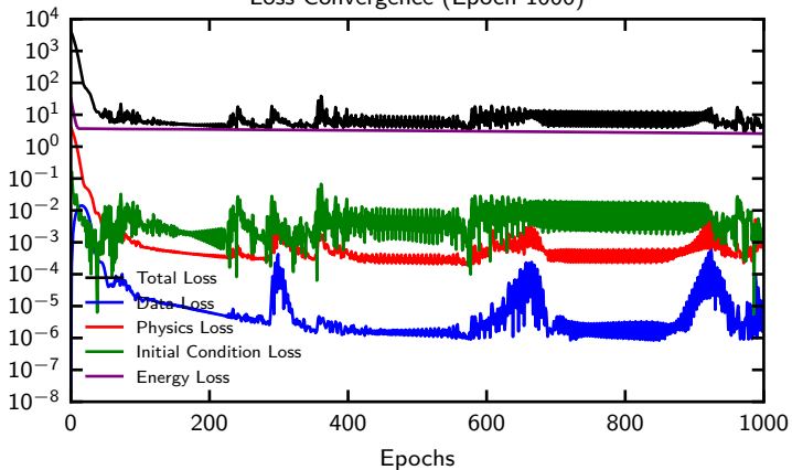
Loss Convergence (Epoch 1000)
