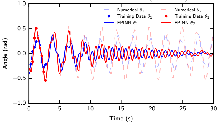
Double Pendulum - Time Domain (Epoch 1000)
