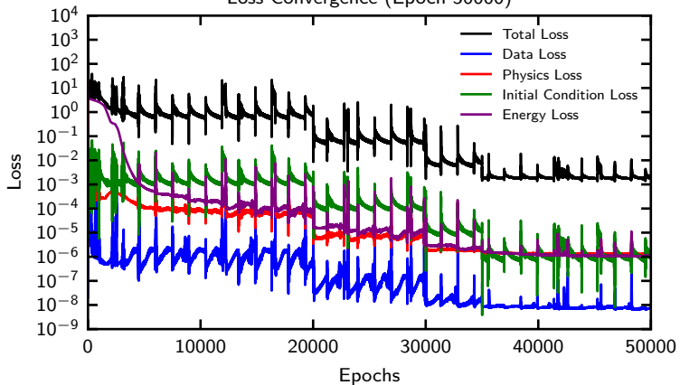
Loss Convergence (Epoch 50000)
