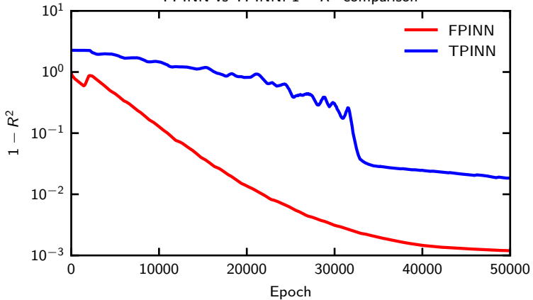
FPINN vs TPINN: 1 - R^2 comparison
