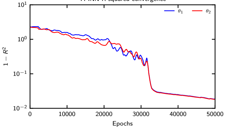
TPINN R-squared convergence
