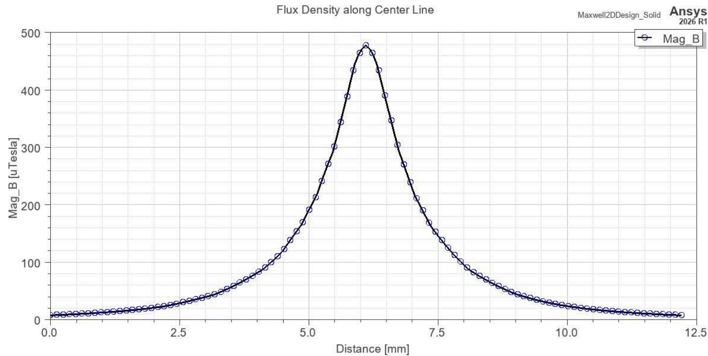
Fig.10 Flux Density along Center Line
