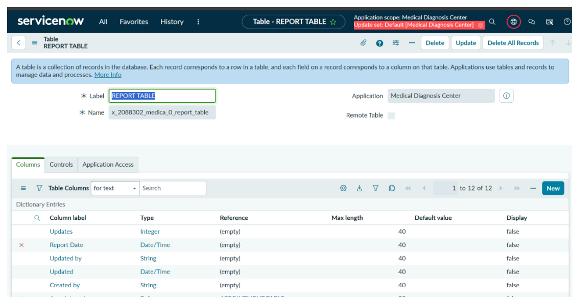
Figure 11: Report Table
