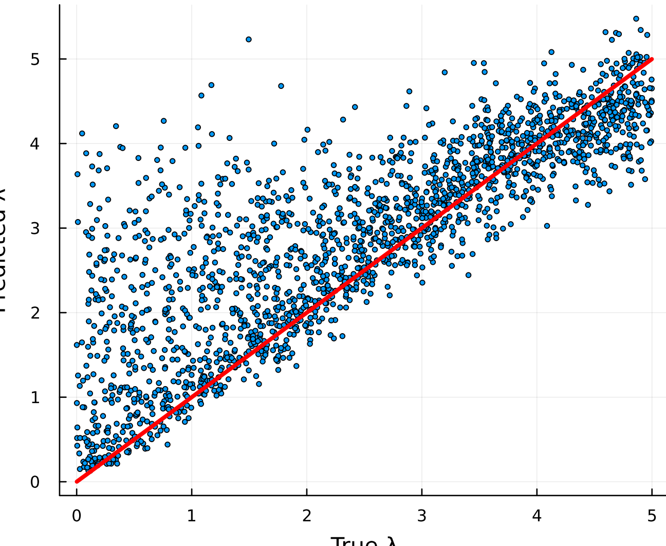
True vs Predicted \lambda
