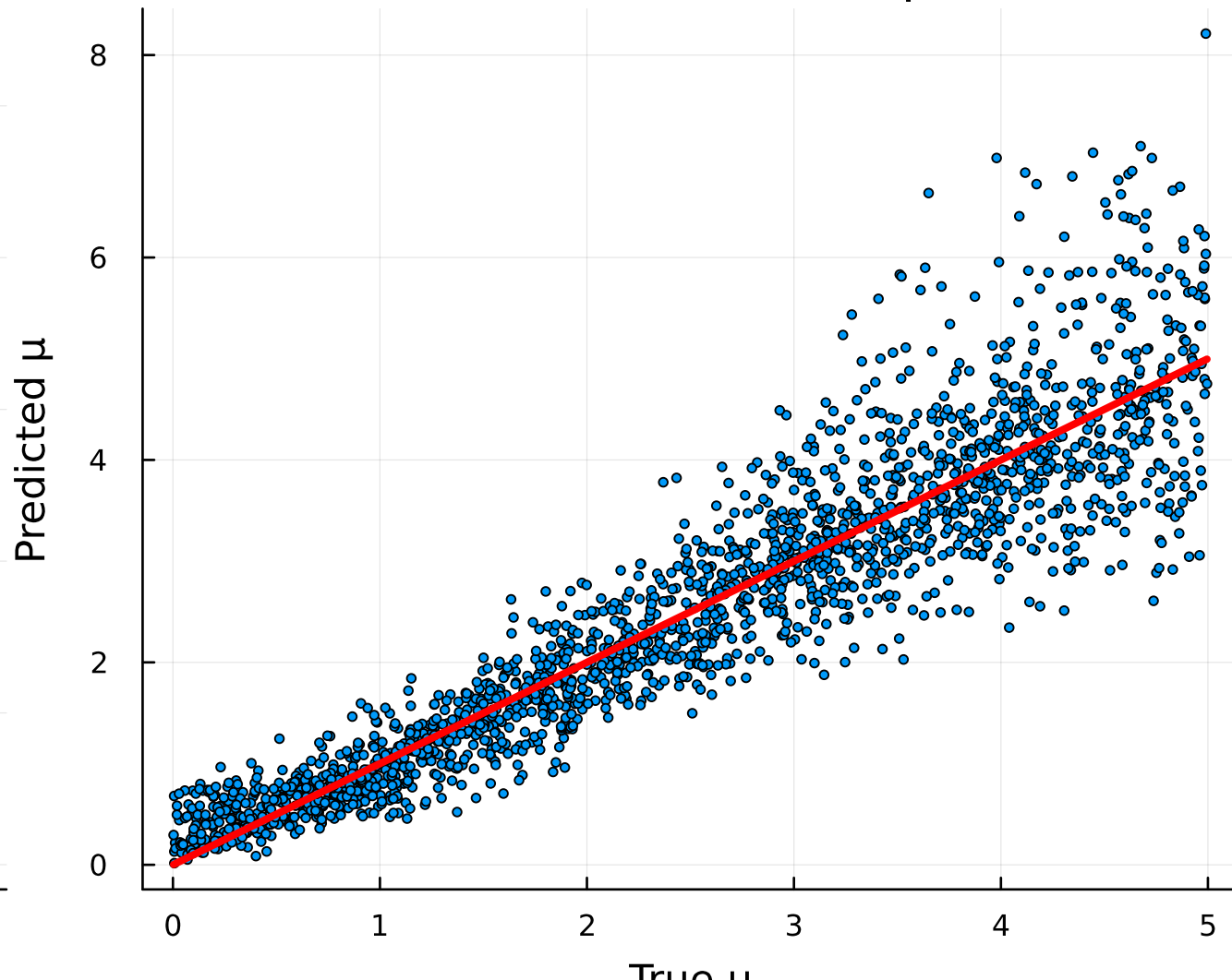
True vs Predicted \mu
