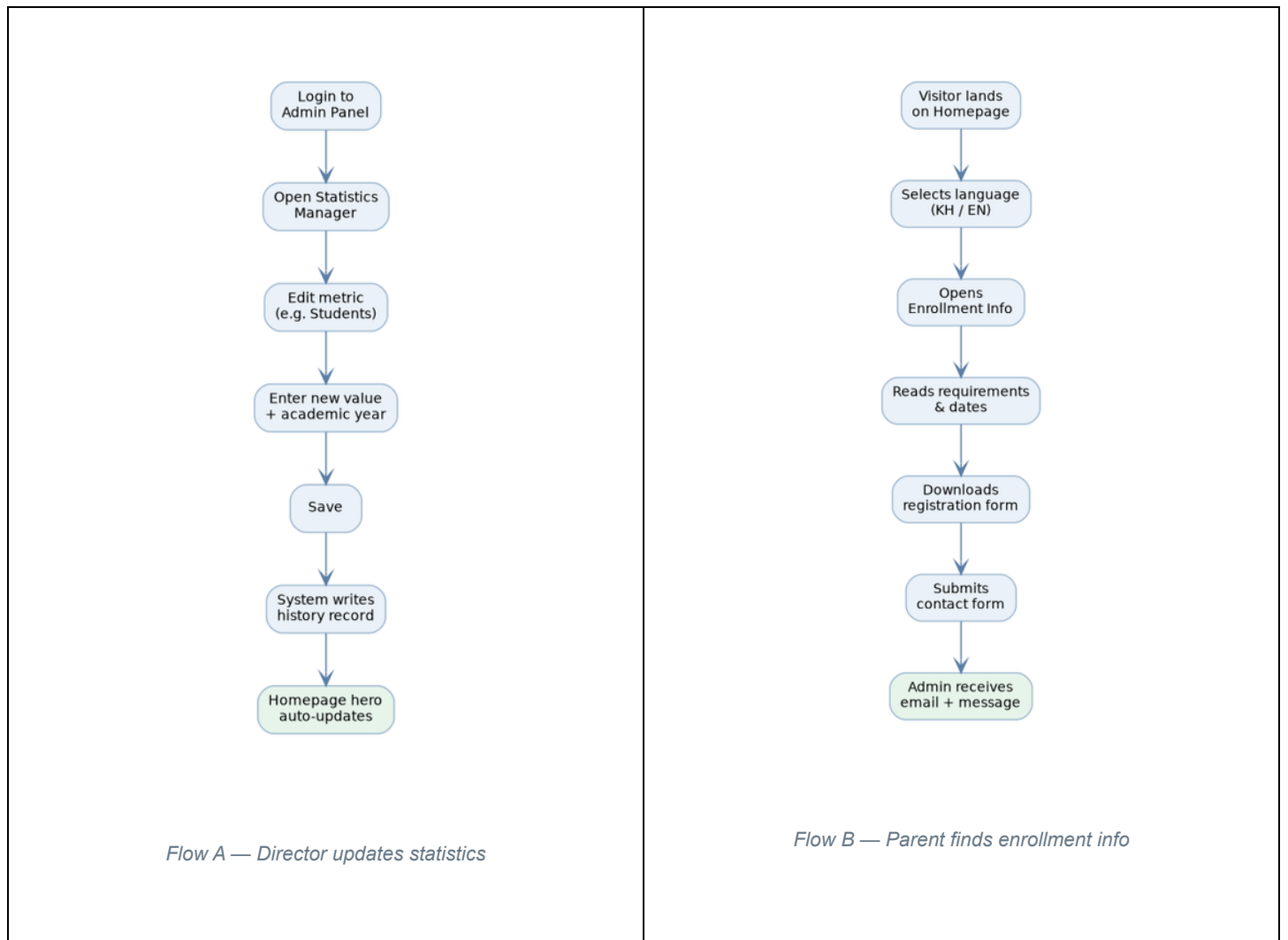
Figure 4 — Representative user flows
