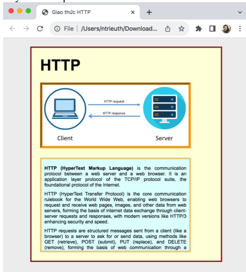
Figure 1. HTTP Protocol
