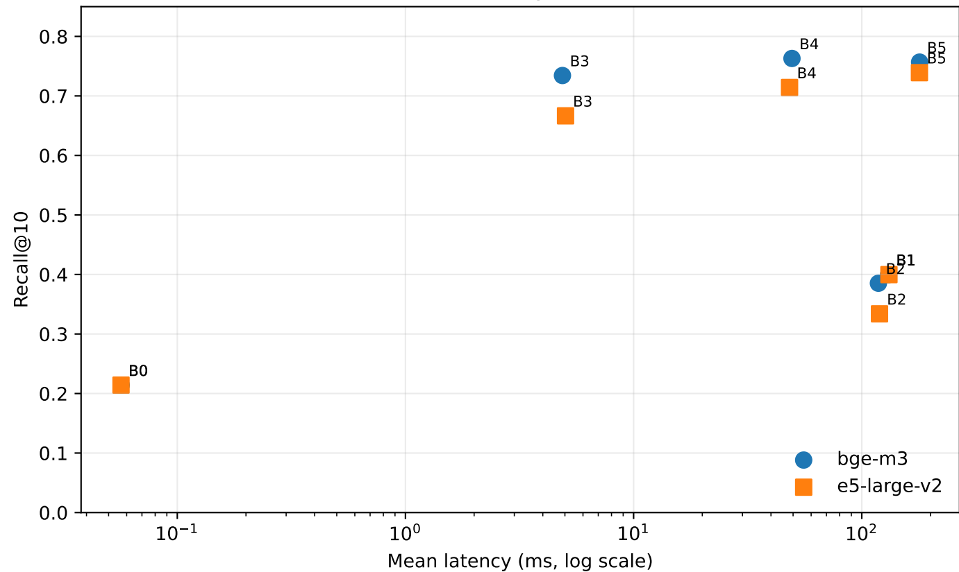
Recall-Latency Trade-off
