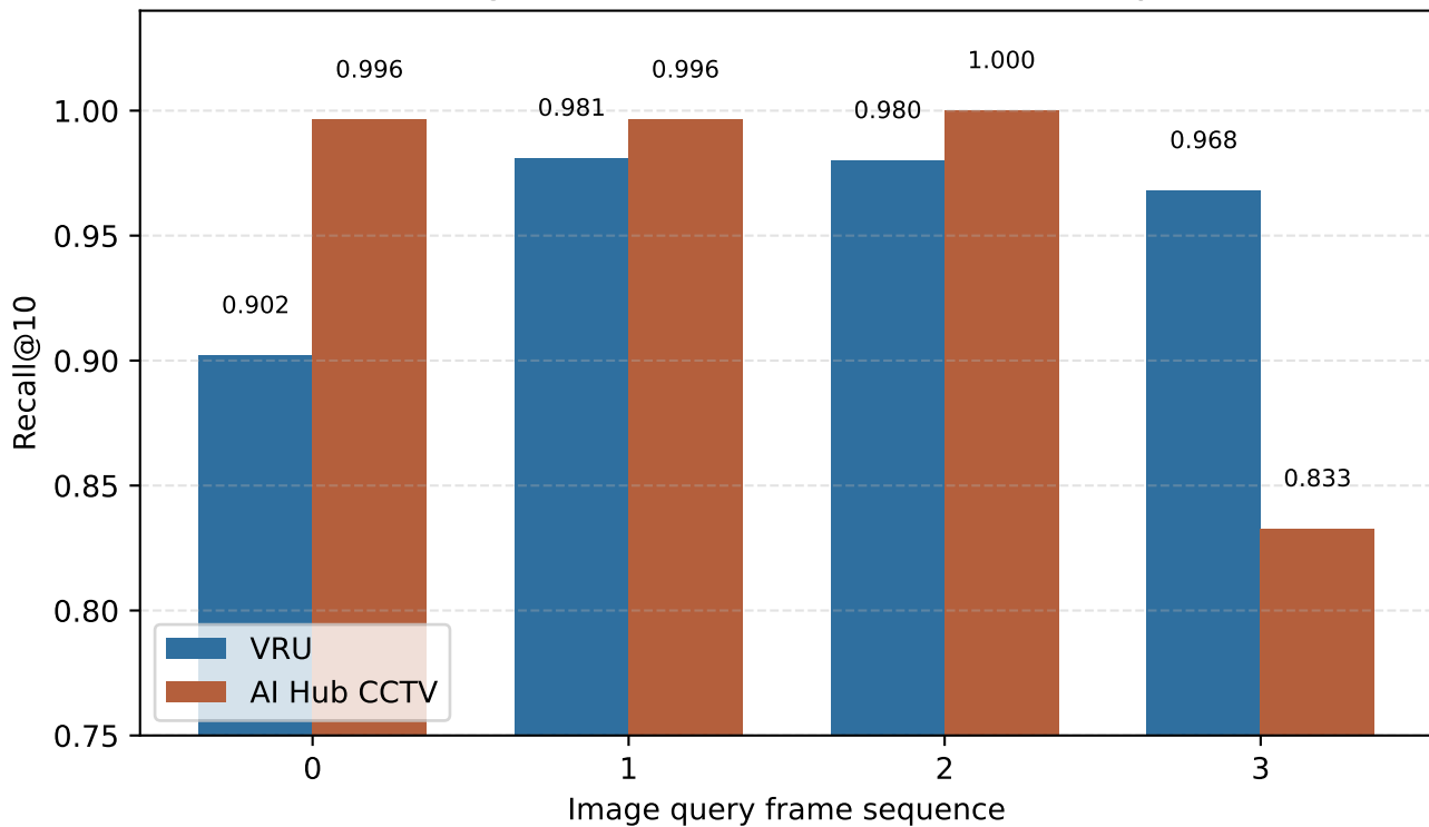
Image-to-Video Frame Position Sensitivity
