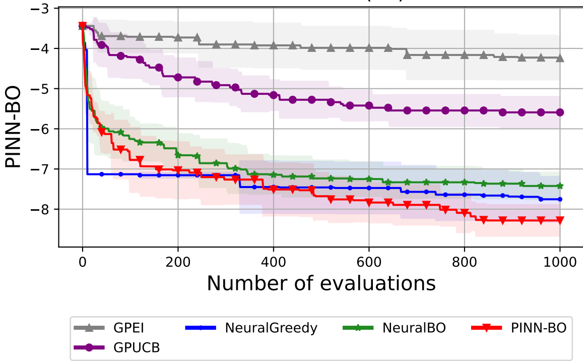
Michalewics (30)
