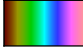
eos b
