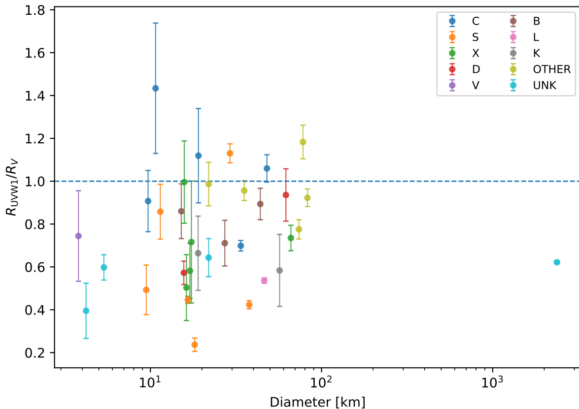
Solar-normalised UVW1 reflectance versus diameter
