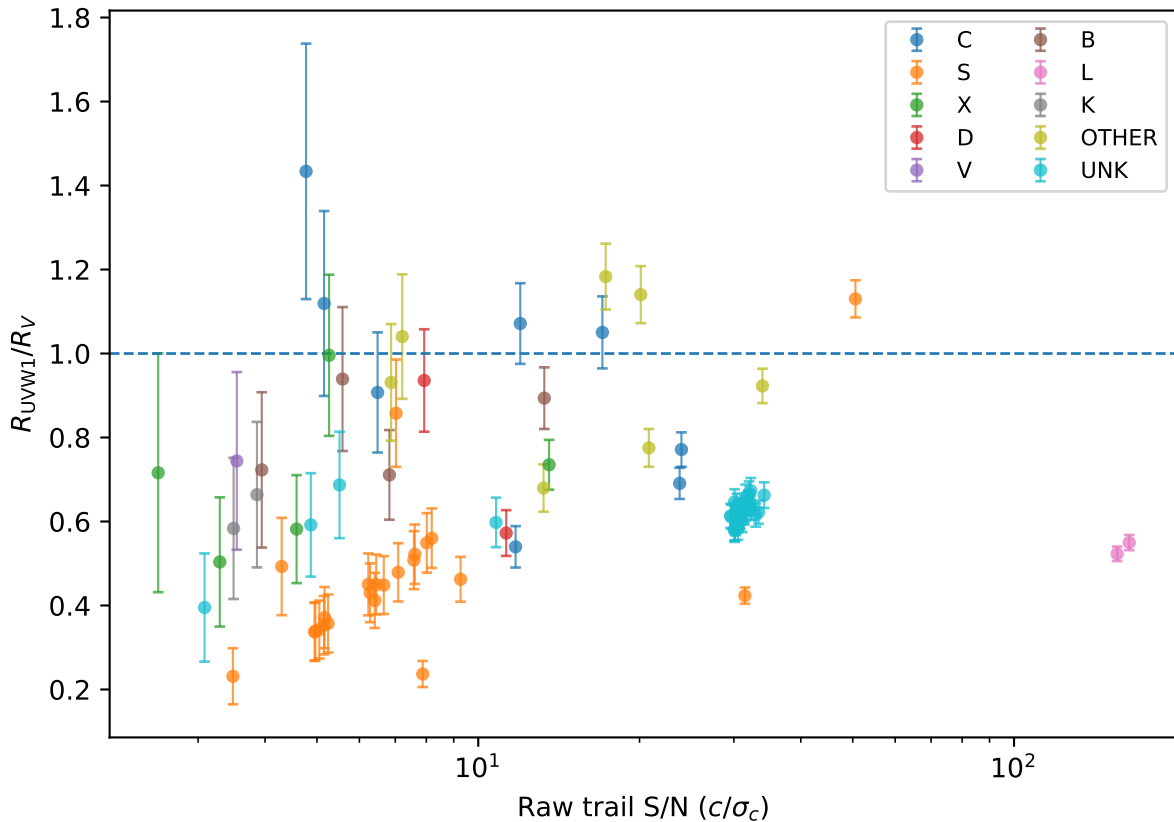
Frame-level UVW1 reflectance versus detection S/N
