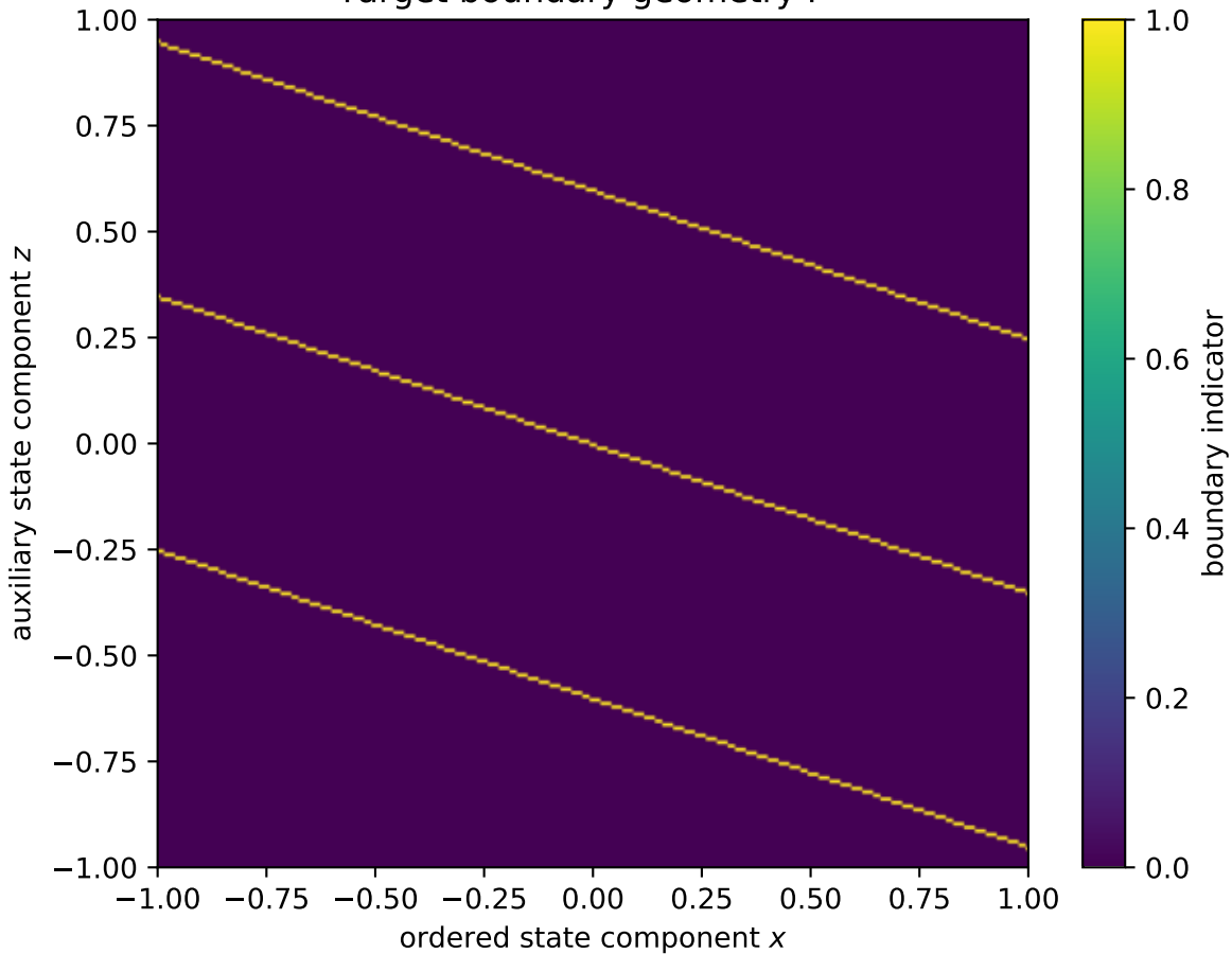
Target boundary geometry \Gamma^*
