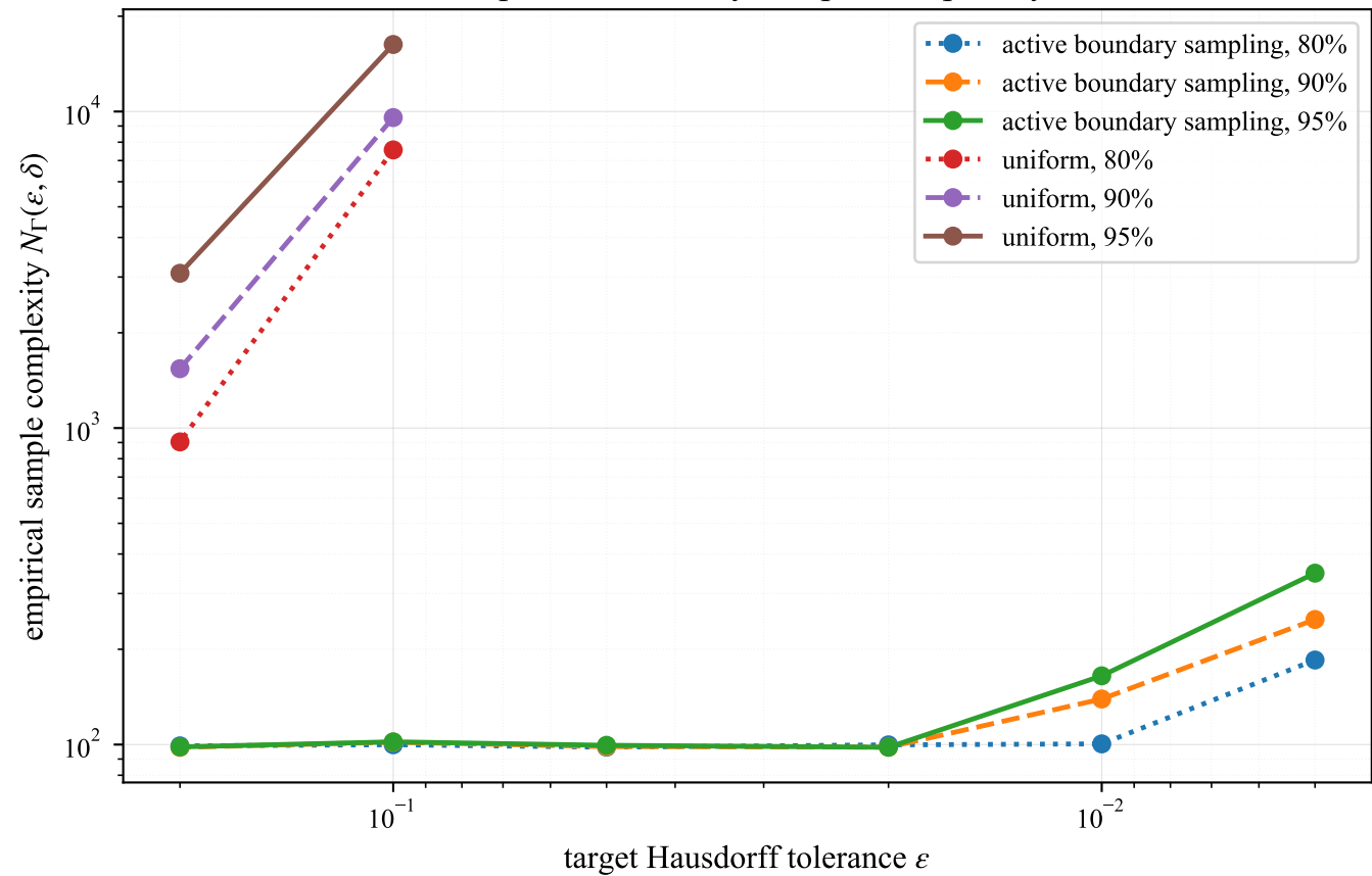
Empirical boundary sample complexity
