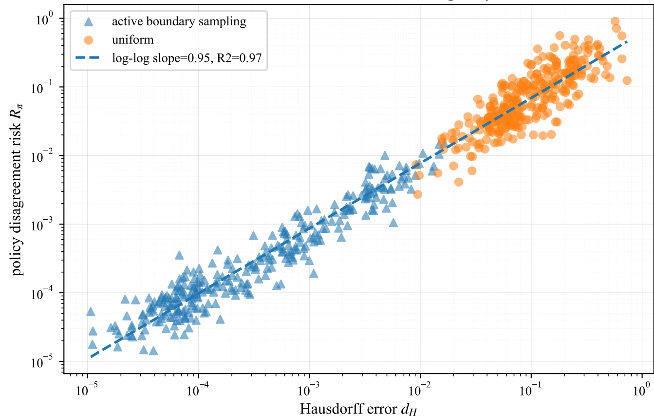
Geometric estimation error controls policy error
