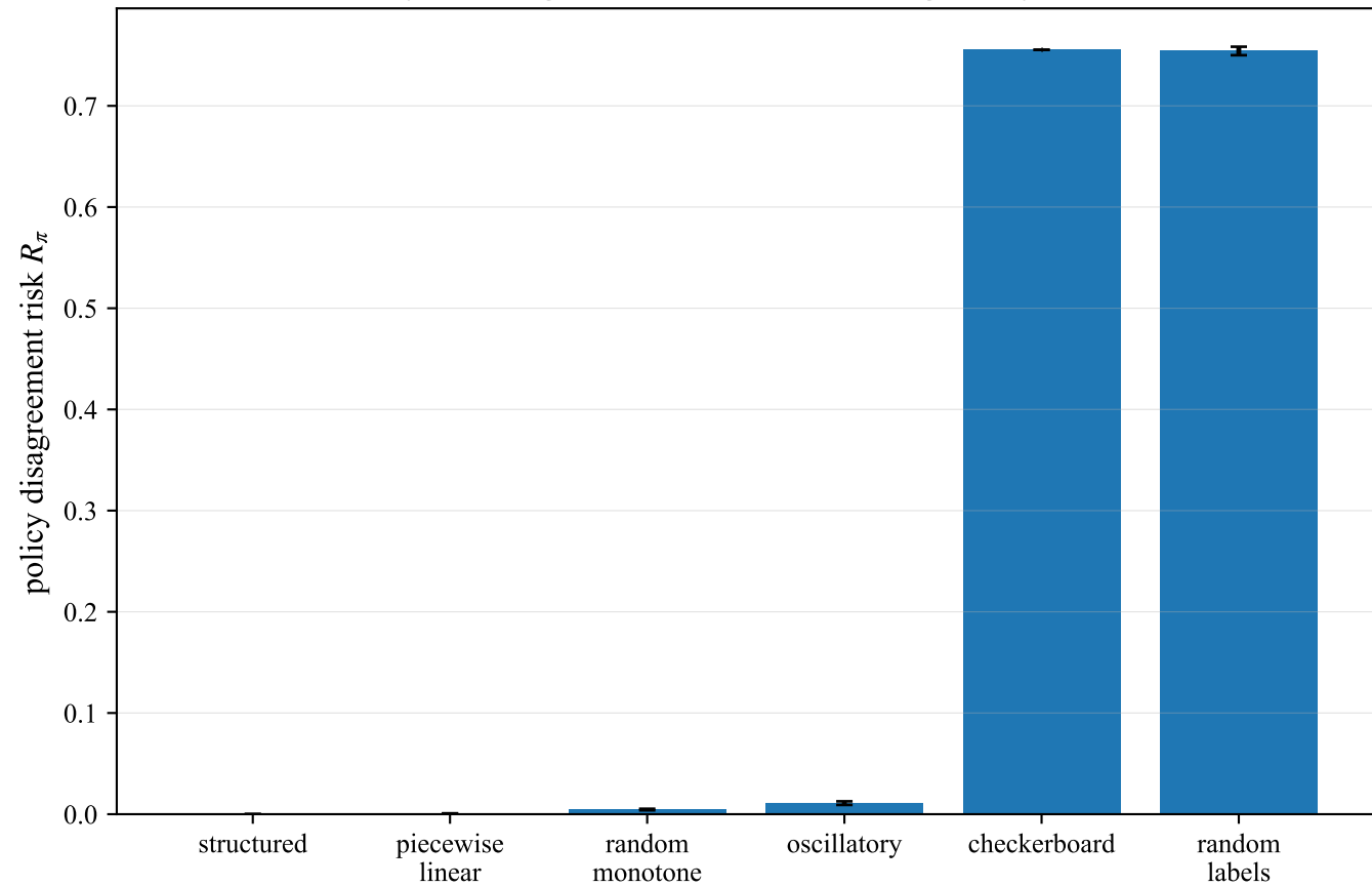
Boundary learning fails when structural regularity is removed
