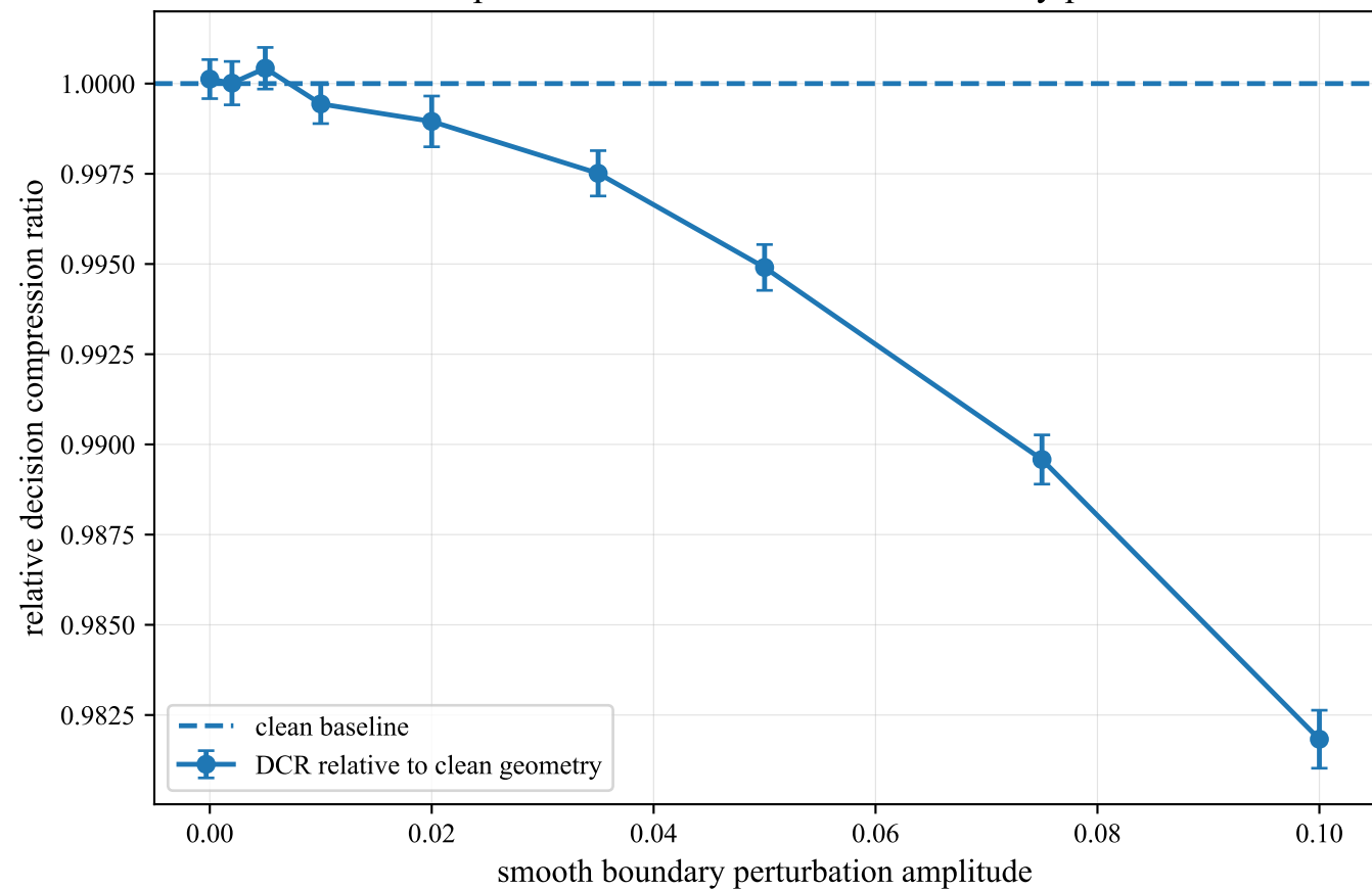
Decision compression is robust to smooth boundary perturbations
