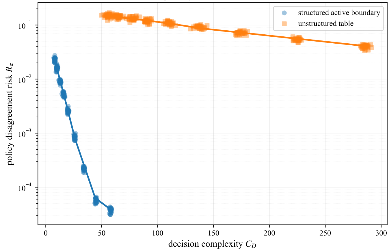
Complexity--risk Pareto frontier
