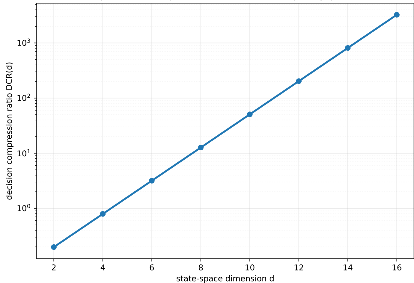
Exponential compression under value complexity growth
